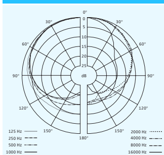
Polar diagram MMD 835-1
