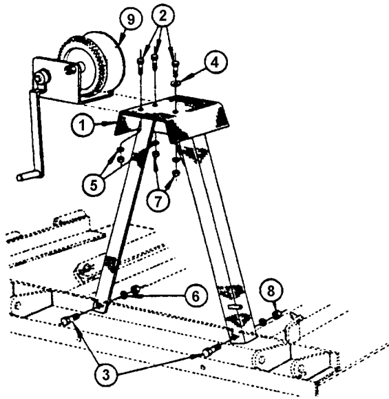
WINCH SUPPORT STAND & SAFETY BRAKE WINCH
