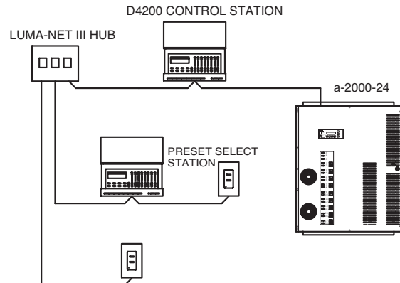
D4200 System Wiring Diagram, Hub
