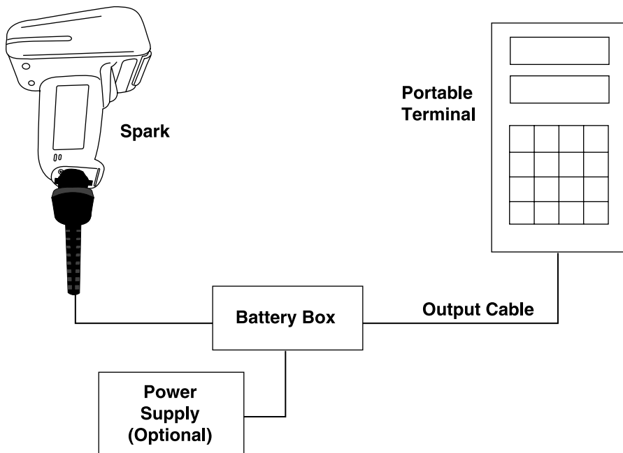
Figure 1-4. RS-232C Operation
