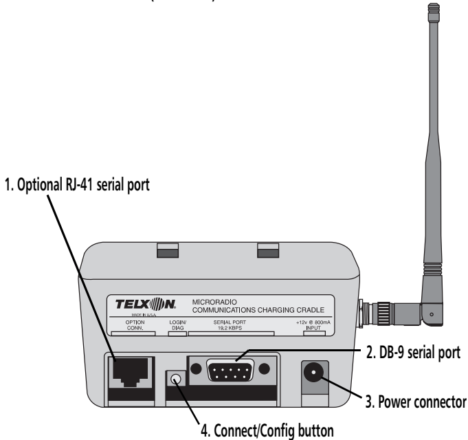
Figure 3. The MRC-921 MicroBase (rear view)
