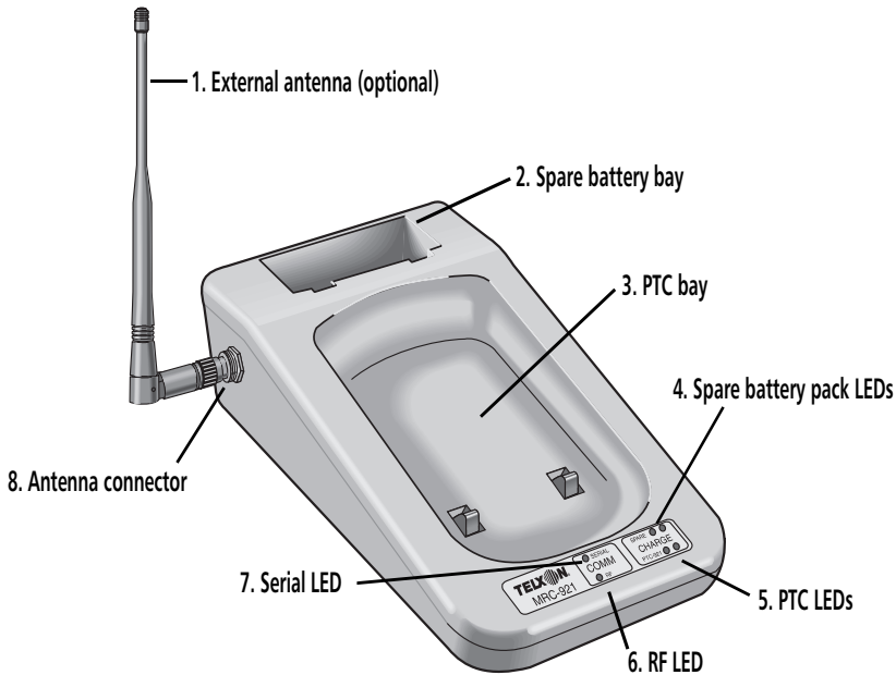
Figure 2. The MRC-921 MicroBase (front view)
