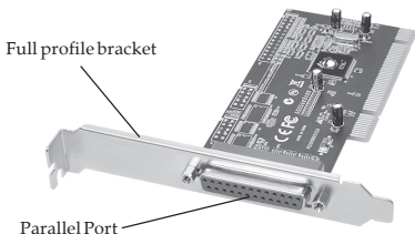
Figure 1: Layout
