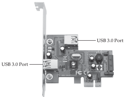
Figure 1: Board Layout
