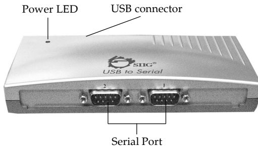
Figure 1. 2-port Layout
