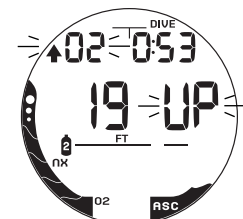
Fig. 87 - O 2 ALARM (after audible)
