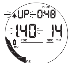
Fig. 83 - HIGH PO2 (during Audible)
