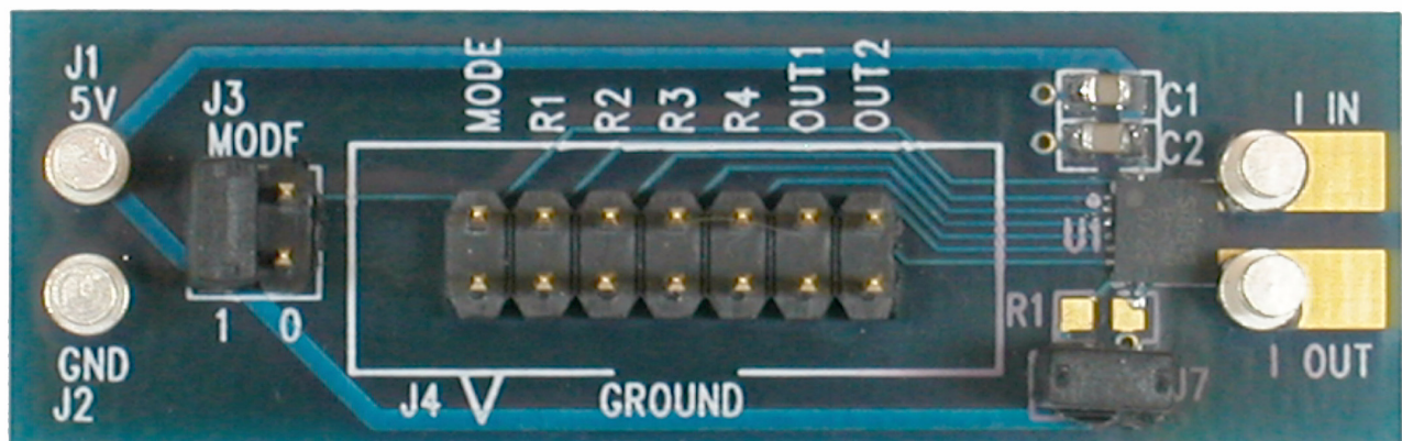
Figure 1. Si85xx-TB Overview
