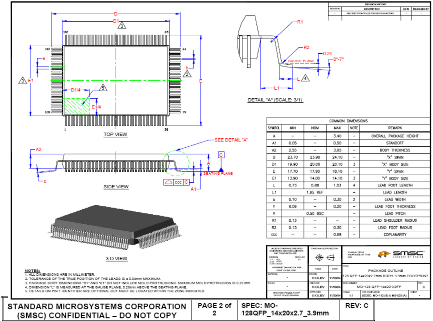
Figure 2 128-Pin QFP Package Outline (3.9mm footprint)
