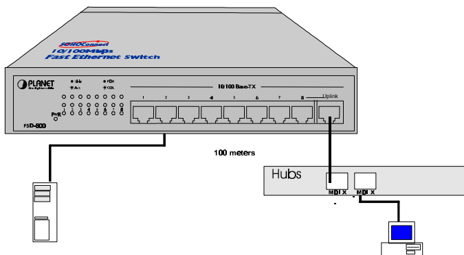
Figure 3. 100Mbps File server to Hubs Connection
