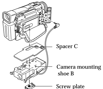
Installation position of the screw plate on the camera mounting shoe B
