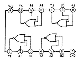
IC355 TC74HC02P
