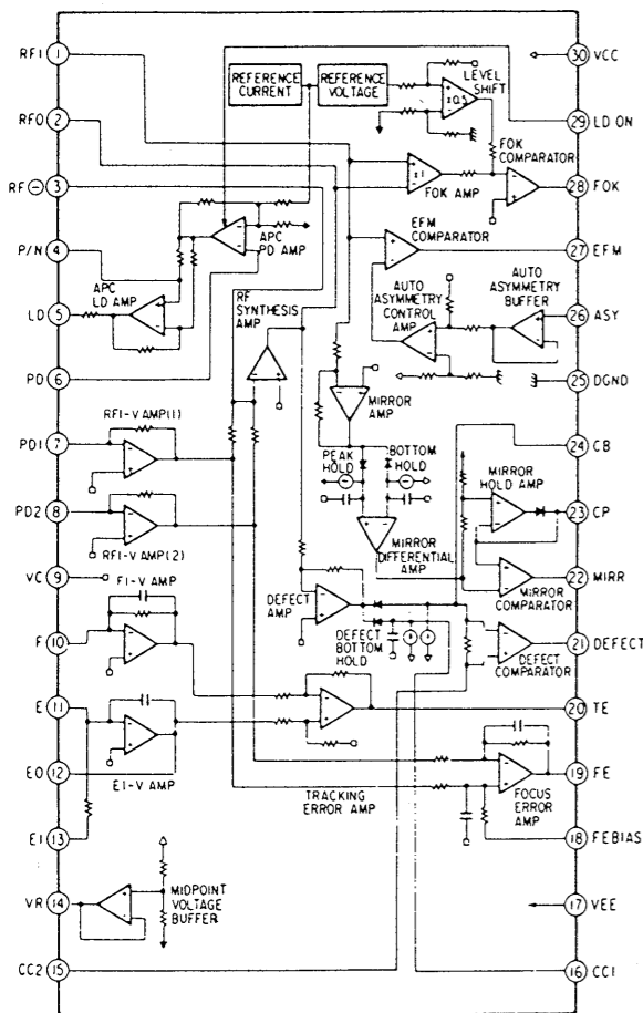
IC101 CXA1081S
