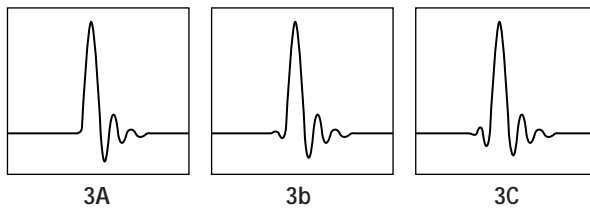
Comparison of filter 3 impulse response
