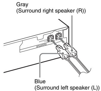
Rear panel of the surround amplifier
