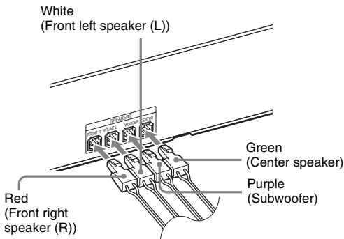
Rear panel of the unit
