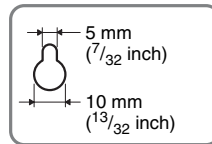
Hole on the back of the speaker
