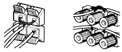
Stripped cords are touching each other due to excessive removal of insulation.
