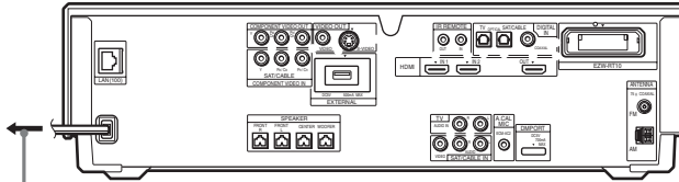
Rear panel of the unit (Ex. BDV-IT1000)
