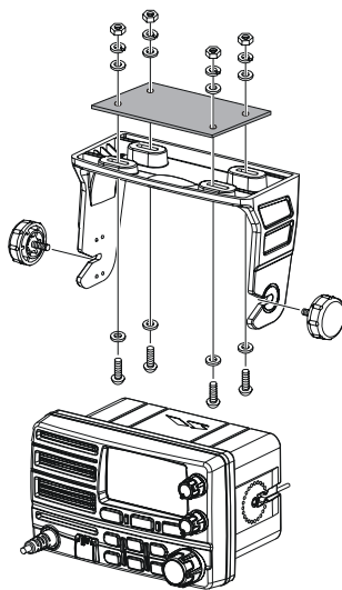
Overhead Mounting
