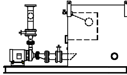
Side View (P2 Pump Shown Only For Clarity)
