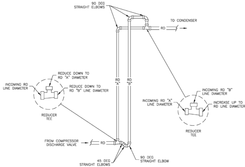
Figure 9: Double Riser Detail
