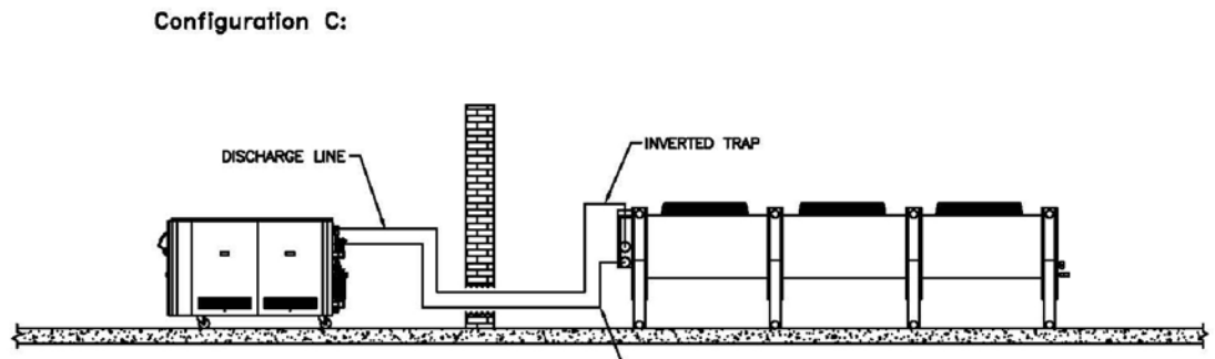
Figure 8: Remote Condenser Configurations
