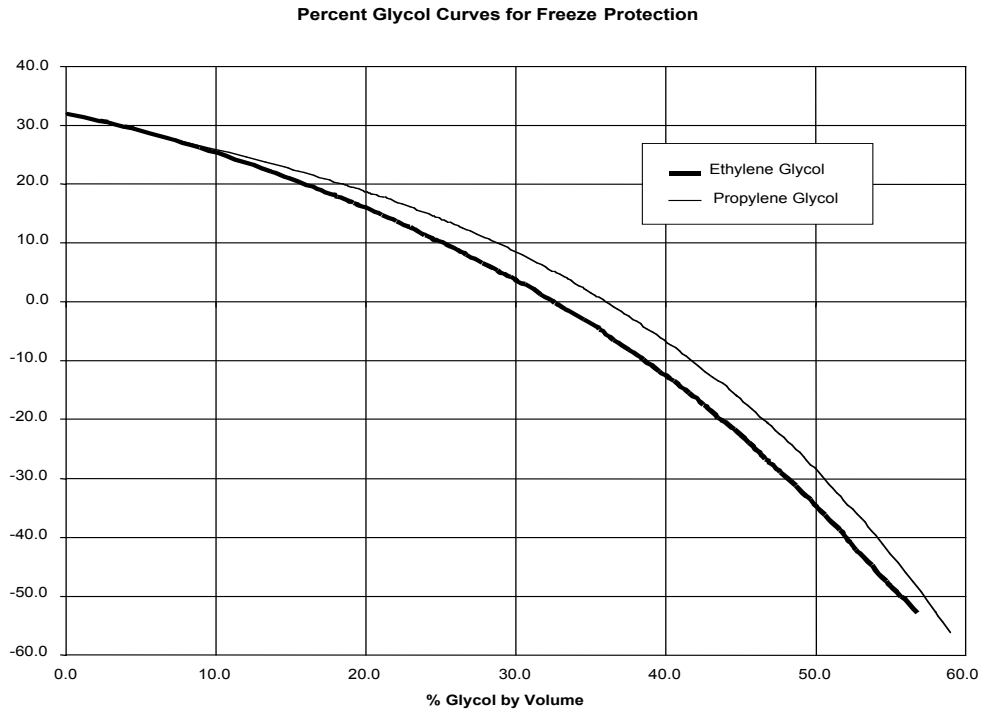
Figure 11: Ethylene Glycol and Propylene Glycol Curves
