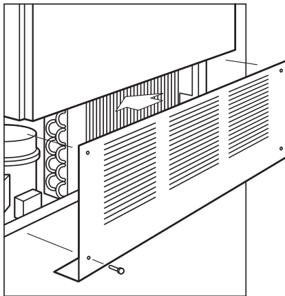
Condenser location
