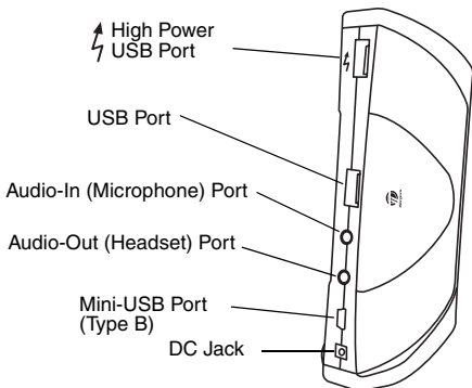
USB 2.0 4-Port Hub Back Vertical View
