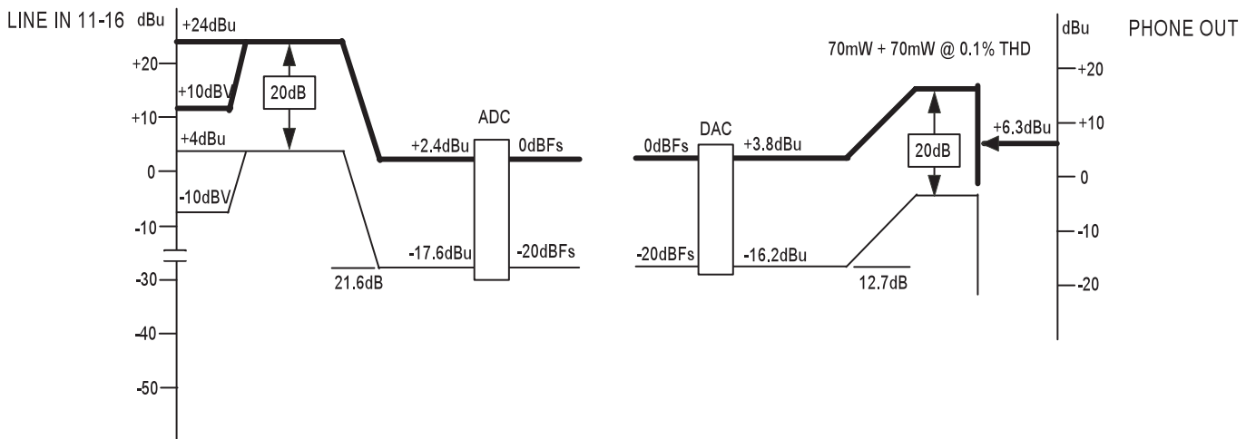
LEVEL DIAGRAM
