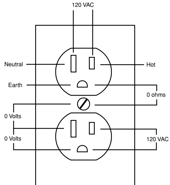
Figure 1. Standard wall Receptacle
