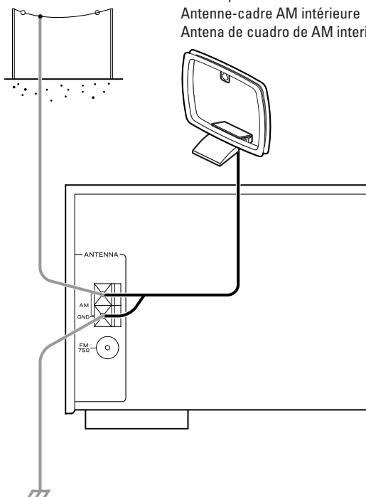
AM Outdoor Antenna Antenne AM extérieure Antena exterior AM
