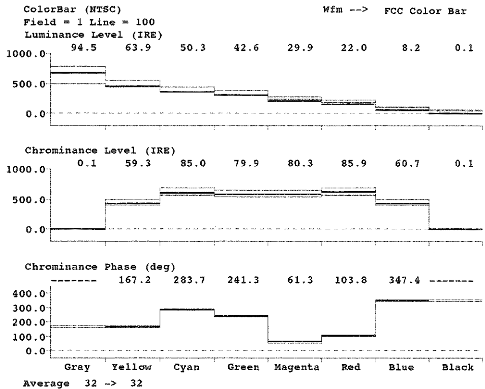
Figure 2-19: ColorBar display
