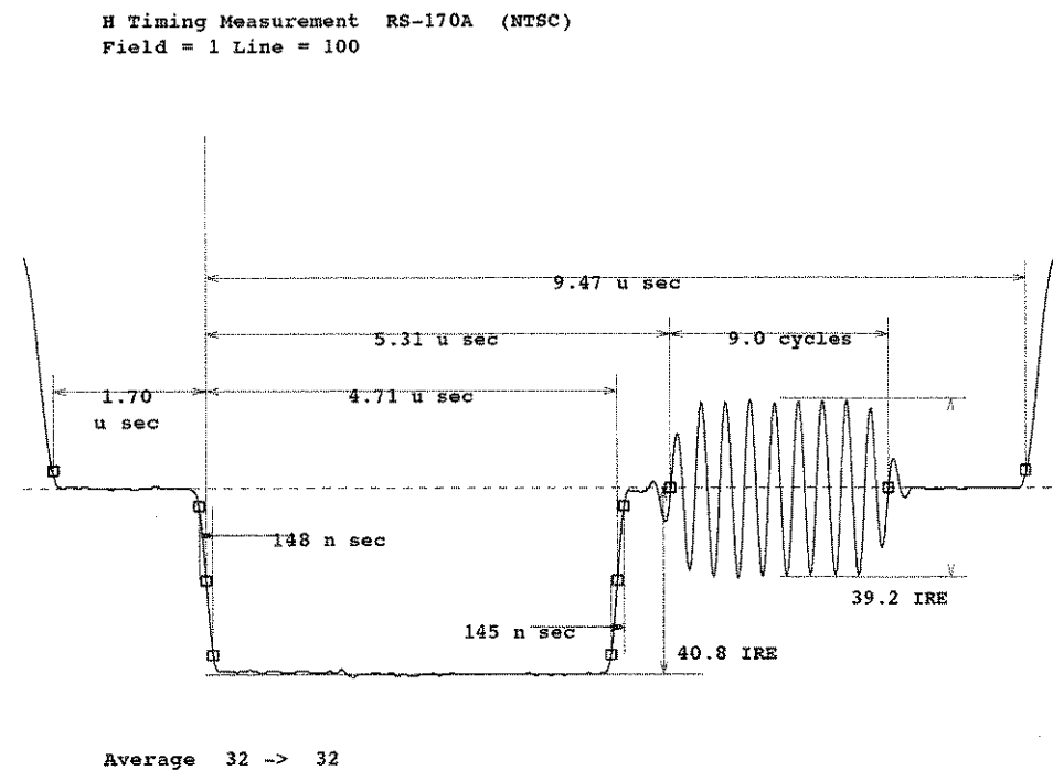
Figure 2-31: H_Timing display
