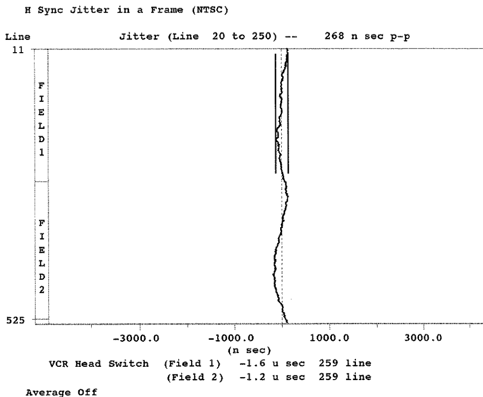
Figure 2-36: Jitter display
