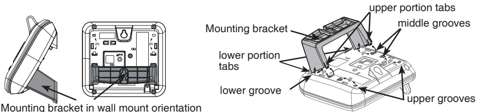
Mounting bracket in wall mount orientation
