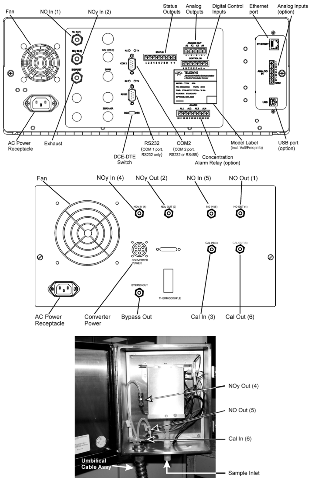
Figure 1. Rear Panels: T200U-NOy Analyzer (top) and 501Y (center); Converter (bottom)
