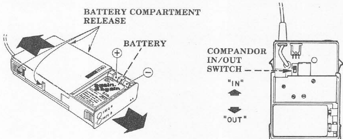
Figure 5 Internal View — WT-400
