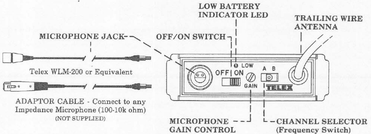
Figure 4 Top Panel — WT-400
