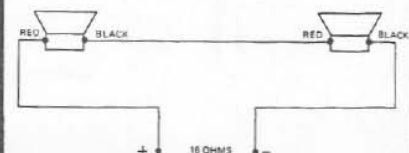
FIGURE 12 Connection of 2 EVM-15L Speakers in Series
