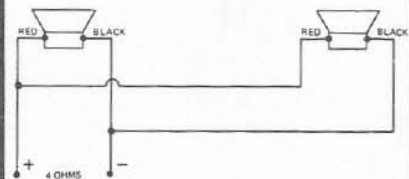
FIGURE 11 Connection of 2 EVM-15L Speakers in Parallel
