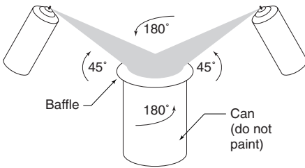
Figure 21: Spray-painting angles
