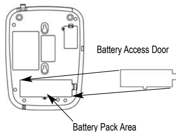
Figure 4 - Battery installation.
