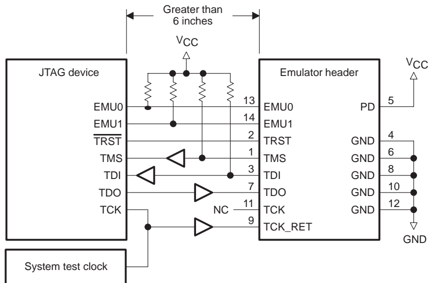
Figure E-6. Target-System-Generated Test Clock
