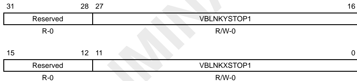
Figure 4–44. Video Display Field 1 Vertical Blanking End Register (VDVBLKE1)
