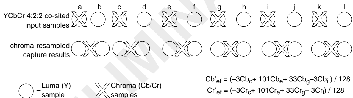
Figure 3–12. Chrominance Resampling
