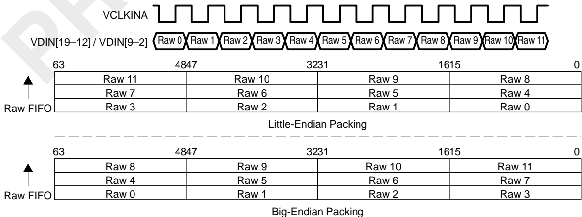
Figure 3–20. 16-Bit Raw Data FIFO Packing
