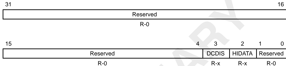
Figure 2–4. Video Port Status Register (VPSTAT)
