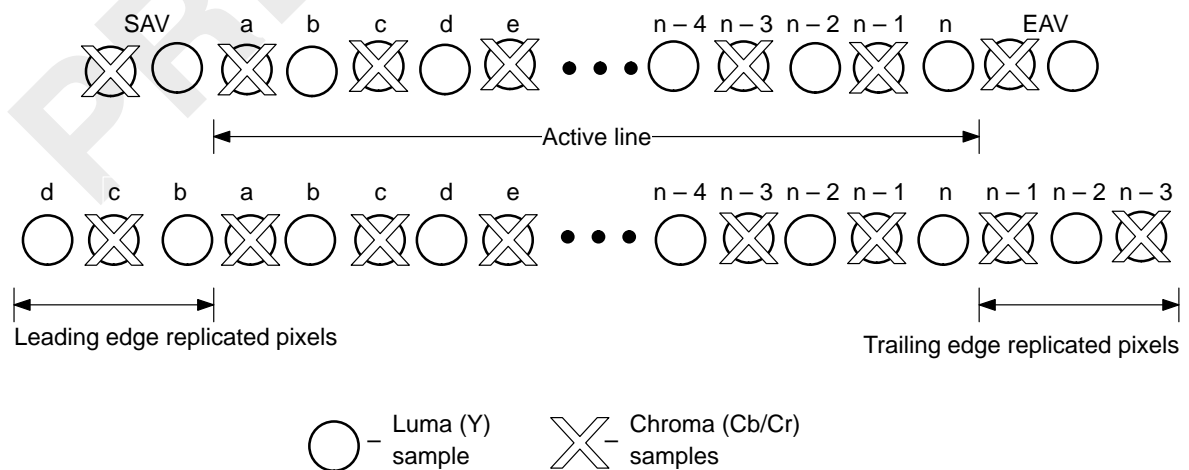
Figure 3–15. Edge Pixel Replication
