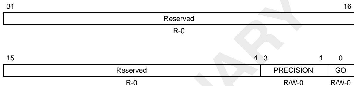
Figure 6–3. VIC Control Register (VICCTL)
