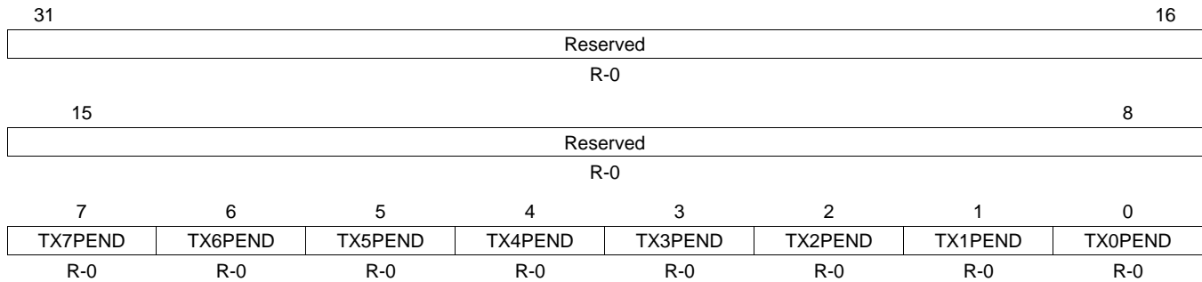
Figure 46. Transmit Interrupt Status (Unmasked) Register (TXINTSTATRAW)
