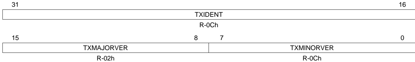
Figure 40. Transmit Identification and Version Register (TXIDVER)
