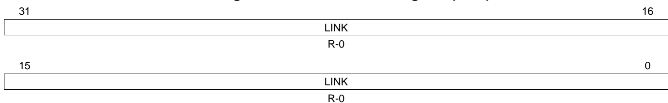
Figure 29. PHY Link Status Register (LINK)
