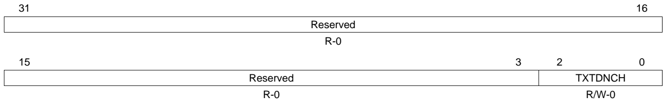
Figure 42. Transmit Teardown Register (TXTEARDOWN)
