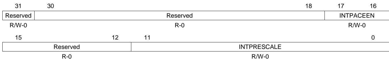
Figure 15. EMAC Control Module Interrupt Control Register (CMINTCTRL)
