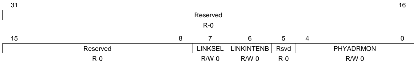
Figure 37. MDIO User PHY Select Register 0 (USERPHYSEL0)
