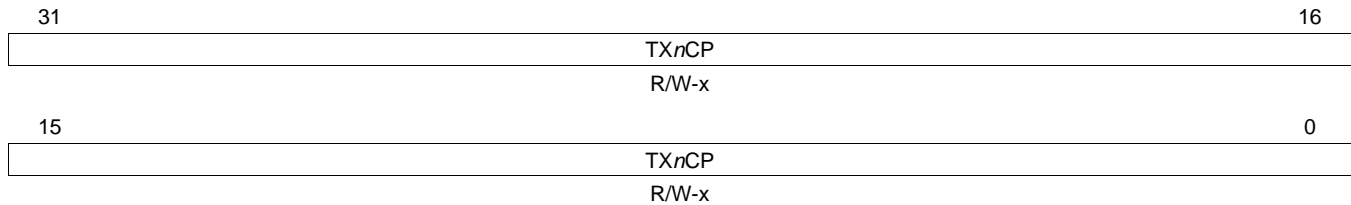
Figure 87. Transmit Channel n Completion Pointer Register (TX n CP)
