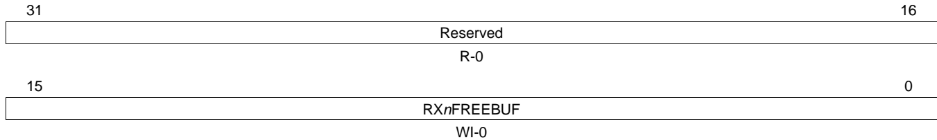
Figure 67. Receive Channel n Free Buffer Count Register (RX n FREEBUFFER)
