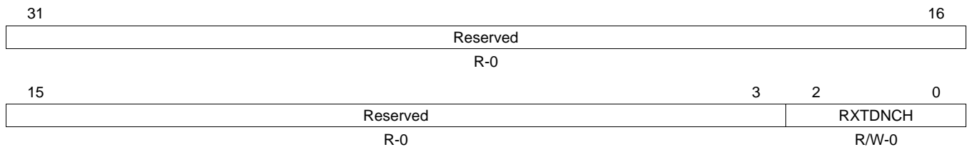
Figure 45. Receive Teardown Register (RXTEARDOWN)
