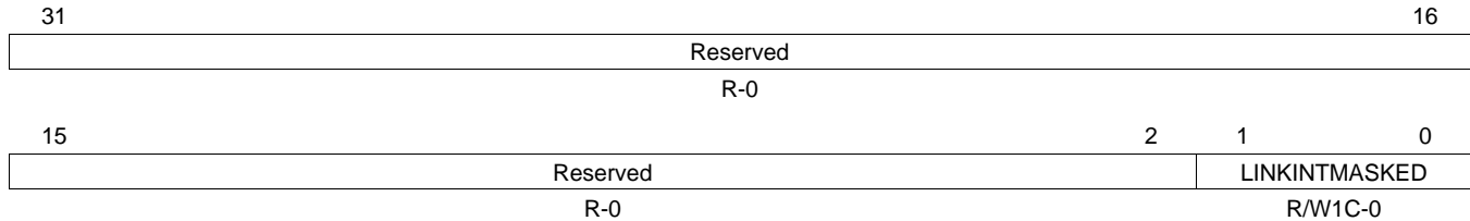
Figure 31. MDIO Link Status Change Interrupt (Masked) Register (LINKINTMASKED)
