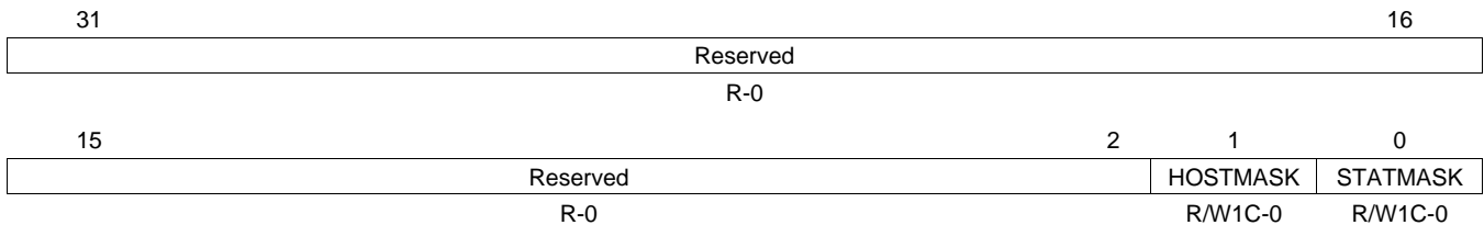
Figure 59. MAC Interrupt Mask Clear Register (MACINTMASKCLEAR)
