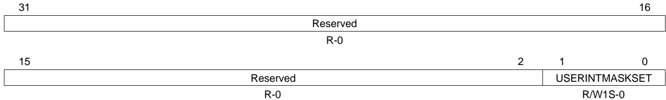
Figure 34. MDIO User Command Complete Interrupt Mask Set Register (USERINTMASKSET)
