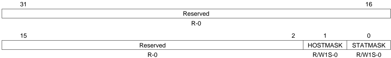
Figure 58. MAC Interrupt Mask Set Register (MACINTMASKSET)
