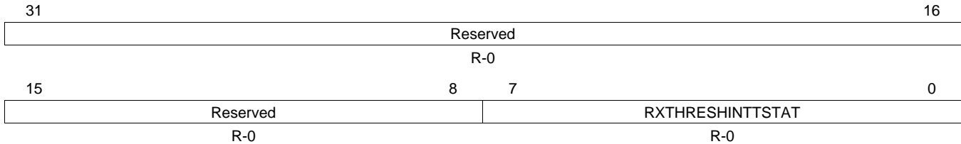
Figure 20. EMAC Control Module Receive Threshold Interrupt Status Register (CMRXTHRESHINTSTAT)
