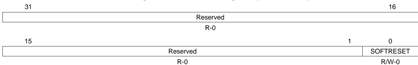
Figure 73. Soft Reset Register (SOFTRESET)
