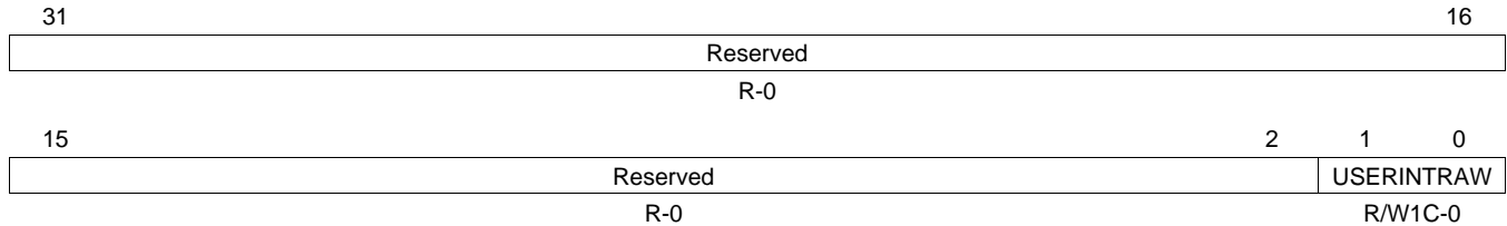
Figure 32. MDIO User Command Complete Interrupt (Unmasked) Register (USERINTRAW)
