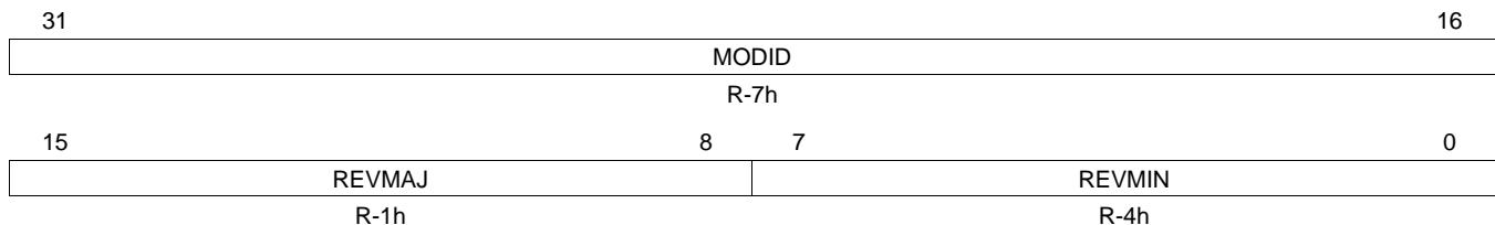
Figure 26. MDIO Version Register (VERSION)
