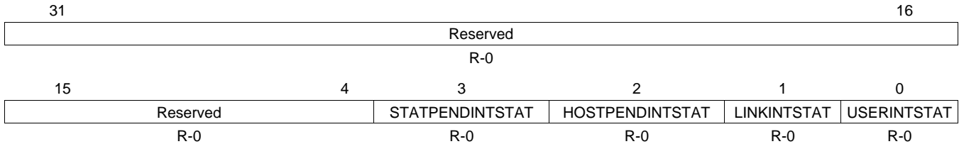
Figure 23. EMAC Control Module Miscellaneous Interrupt Status Register (CMMISCINTSTAT)
