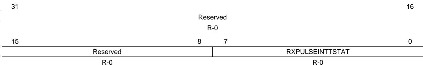
Figure 21. EMAC Control Module Receive Interrupt Status Register (CMRXINTSTAT)
