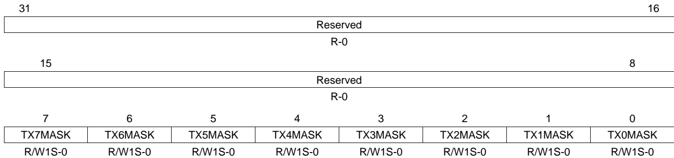
Figure 48. Transmit Interrupt Mask Set Register (TXINTMASKSET)
