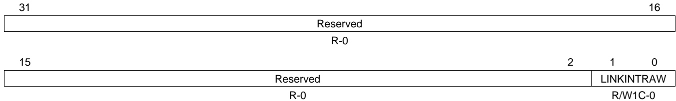
Figure 30. MDIO Link Status Change Interrupt (Unmasked) Register (LINKINTRA \bar{W} )
