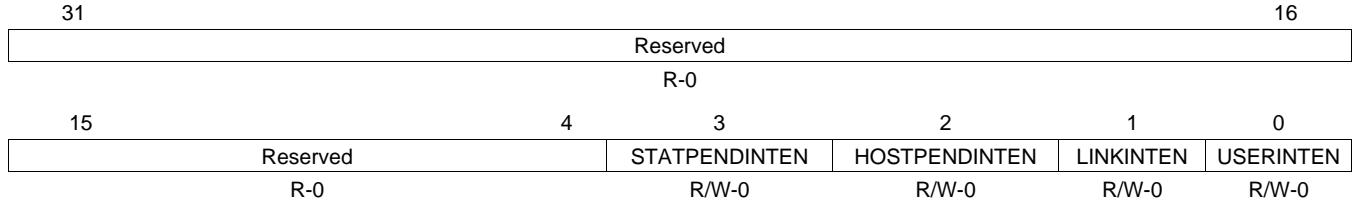
Figure 19. EMAC Control Module Miscellaneous Interrupt Enable Register (CMMISCINTEN)
