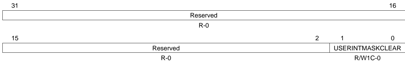
Figure 35. MDIO User Command Complete Interrupt Mask Clear Register (USERINTMASKCLEAR)
