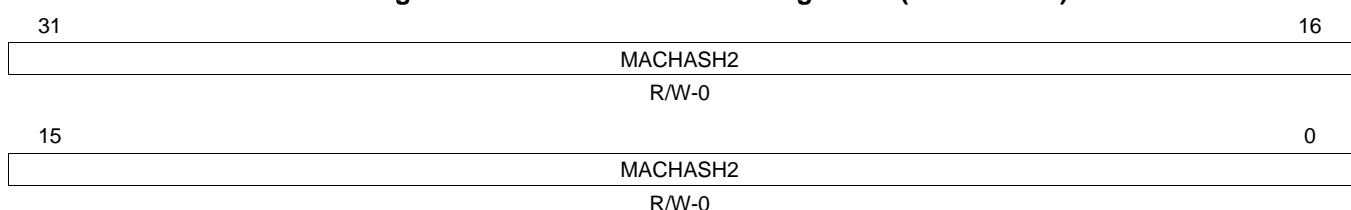
Figure 77. MAC Hash Address Register 2 (MACHASH2)
