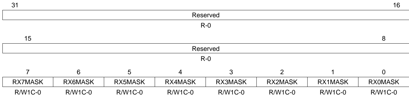
Figure 55. Receive Interrupt Mask Clear Register (RXINTMASKCLEAR)
