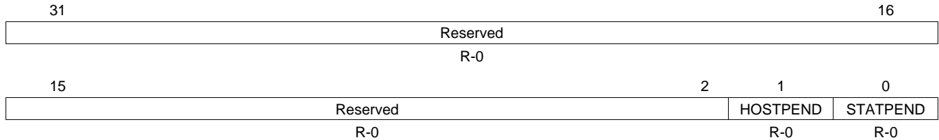
Figure 56. MAC Interrupt Status (Unmasked) Register (MACINTSTATRAW)
