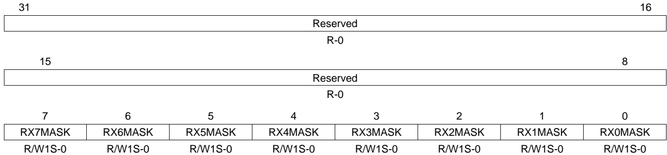
Figure 54. Receive Interrupt Mask Set Register (RXINTMASKSET)
