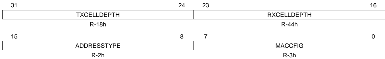
Figure 72. MAC Configuration Register (MACCONFIG)
