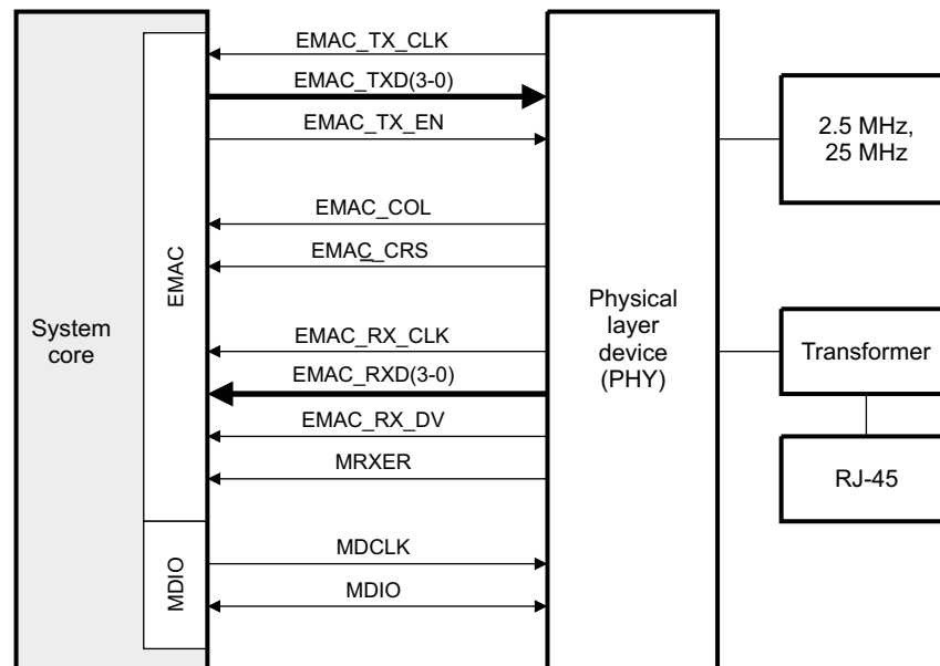
Figure 2. Ethernet Configuration MII Connections
