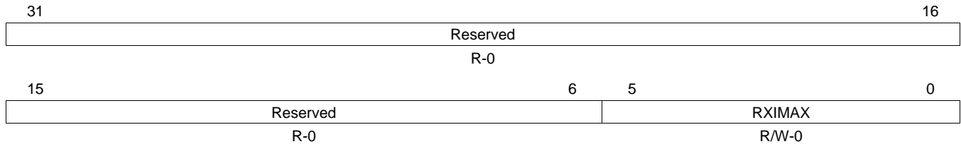
Figure 24. EMAC Control Module Receive Interrupts per Millisecond Register (CMRXINTMAX)
