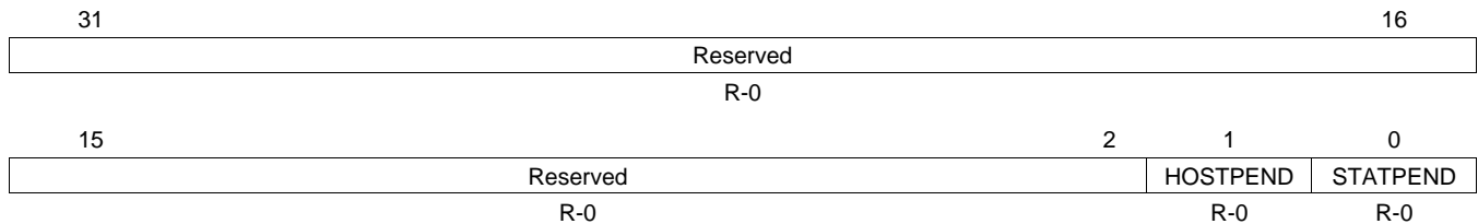
Figure 57. MAC Interrupt Status (Masked) Register (MACINTSTATMASKED)
