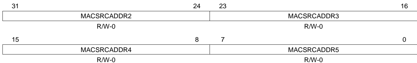
Figure 75. MAC Source Address High Bytes Register (MACSRCADDRHI)
