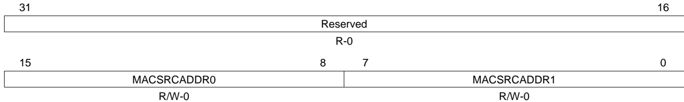
Figure 74. MAC Source Address Low Bytes Register (MACSRCADDRLO)
