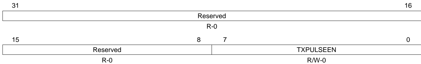
Figure 18. EMAC Control Module Transmit Interrupt Enable Register (CMTXINTEN)
