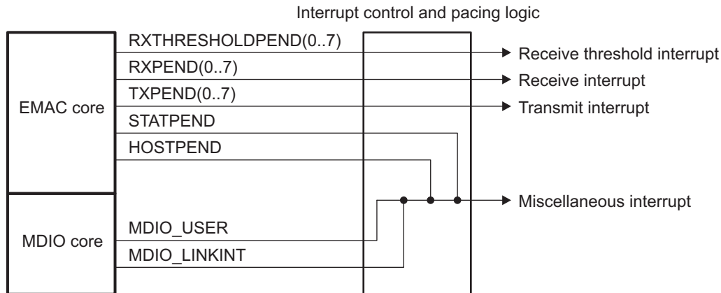
Figure 11. EMAC Control Module Interrupt Logic Diagram
