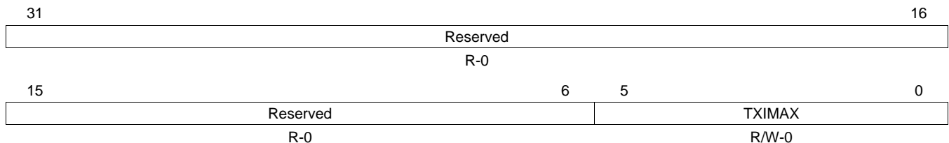
Figure 25. EMAC Control Module Transmit Interrupts per Millisecond Register (CMTXINTMAX)
