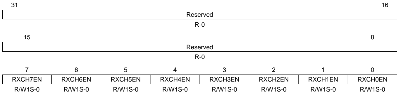
Figure 61. Receive Unicast Enable Set Register (RXUNICASTSET)
