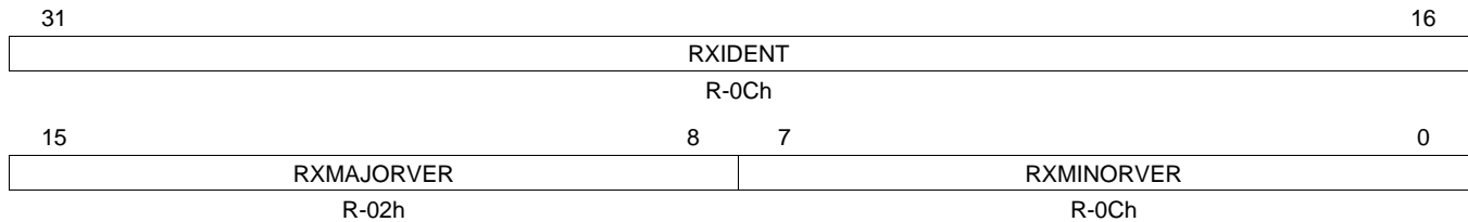
Figure 43. Receive Identification and Version Register (RXIDVER)
