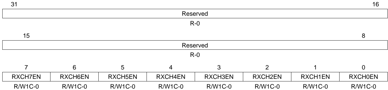
Figure 62. Receive Unicast Clear Register (RXUNICASTCLEAR)
