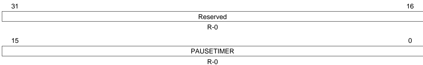
Figure 81. Transmit Pause Timer Register (TXPAUSE)
