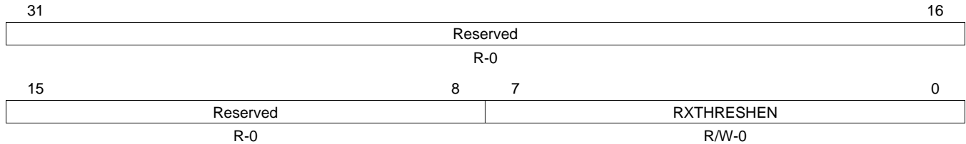
Figure 16. EMAC Control Module Receive Threshold Interrupt Enable Register (CMRXTHRESHINTEN)
