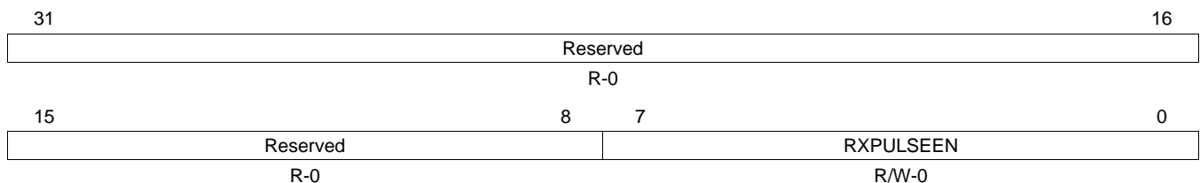
Figure 17. EMAC Control Module Receive Interrupt Enable Register (CMRXINTEN)
