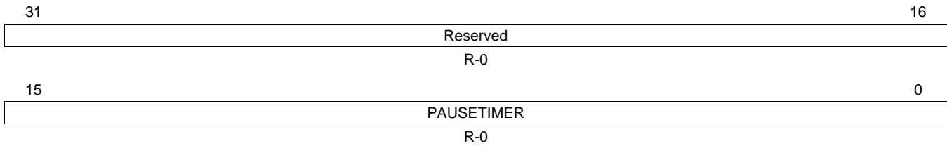
Figure 80. Receive Pause Timer Register (RXPAUSE)
