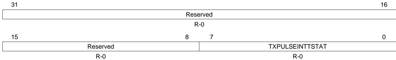
Figure 22. EMAC Control Module Transmit Interrupt Status Register (CMTXINTSTAT)
