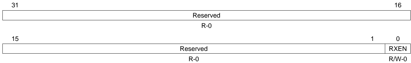
Figure 44. Receive Control Register (RXCONTROL)
