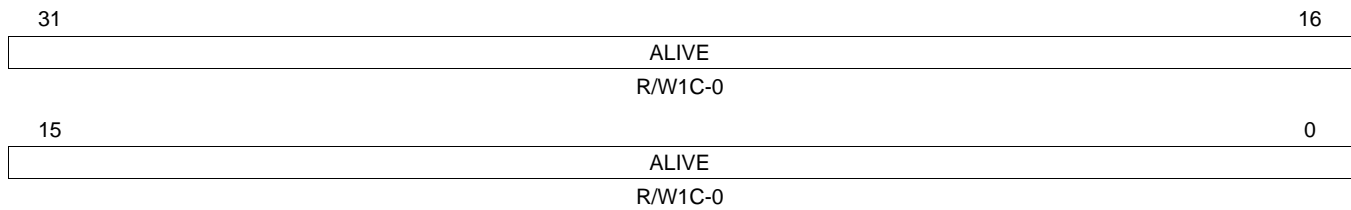
Figure 28. PHY Acknowledge Status Register (ALIVE)
