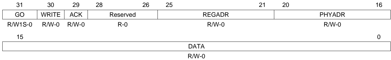
Figure 36. MDIO User Access Register 0 (USERACCESS0)
