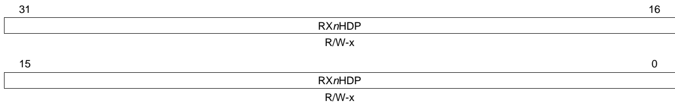
Figure 86. Receive Channel n DMA Head Descriptor Pointer Register (RXnHDP)
