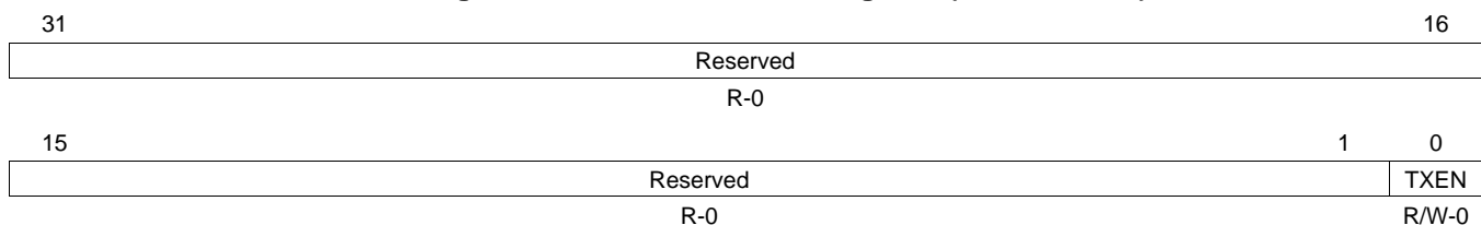
Figure 41. Transmit Control Register (TXCONTROL)
