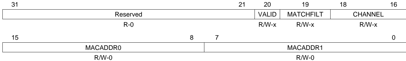
Figure 82. MAC Address Low Bytes Register (MACADDRLO)
