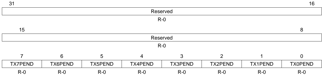
Figure 45. Transmit Interrupt Status (Unmasked) Register (TXINTSTATRAW)
