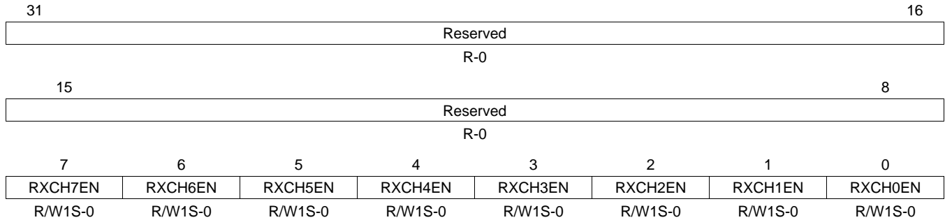
Figure 60. Receive Unicast Enable Set Register (RXUNICASTSET)
