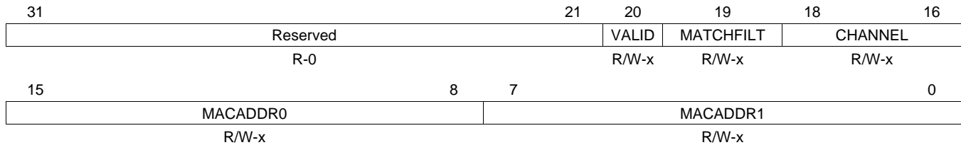
Figure 81. MAC Address Low Bytes Register (MACADDRLO)
