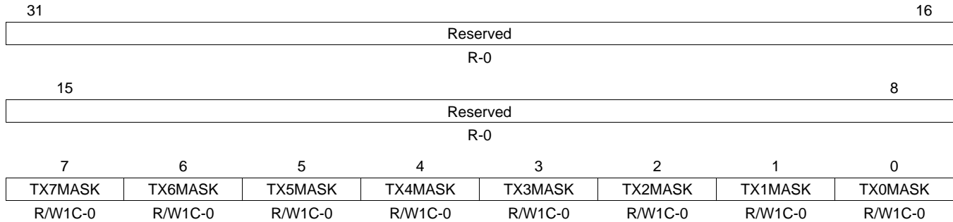
Figure 48. Transmit Interrupt Mask Clear Register (TXINTMASKCLEAR)
