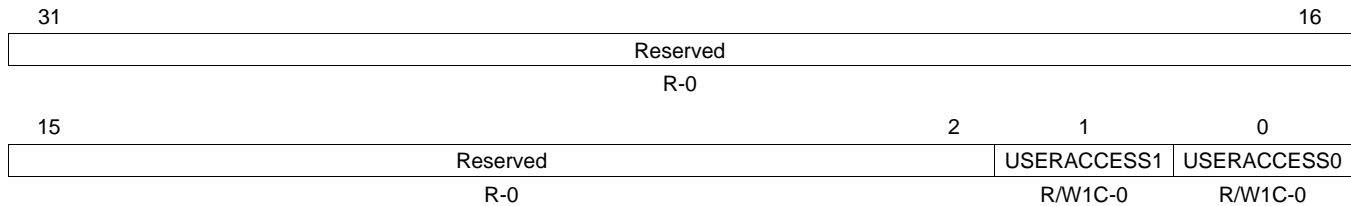
Figure 34. MDIO User Command Complete Interrupt Mask Clear Register (USERINTMASKCLEAR)
