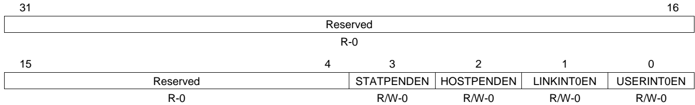
Figure 18. EMAC Control Module Interrupt Core 0-2 Miscellaneous Interrupt Enable Register (CnMISCEN)
