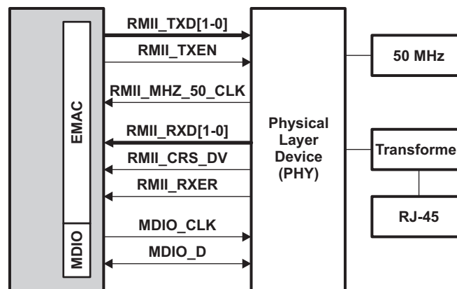
Figure 3. Ethernet Configuration—RMII Connections
