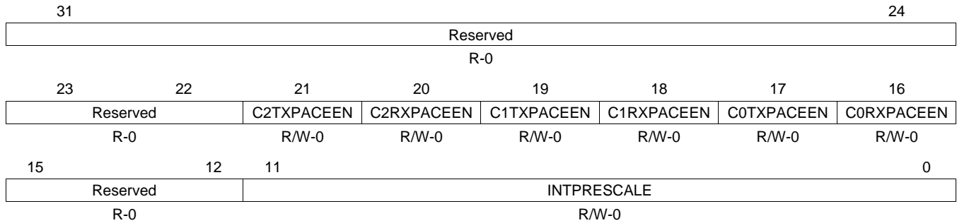
Figure 14. EMAC Control Module Interrupt Control Register (INTCONTROL)
