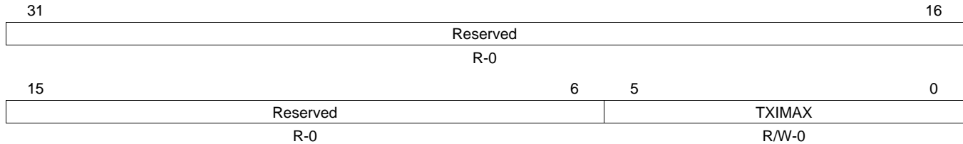
Figure 24. EMAC Control Module Interrupt Core 0-2 Transmit Interrupts Per Millisecond Register (CnTXIMAX)
