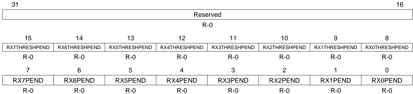
Figure 52. Receive Interrupt Status (Masked) Register (RXINTSTATMASKED)
