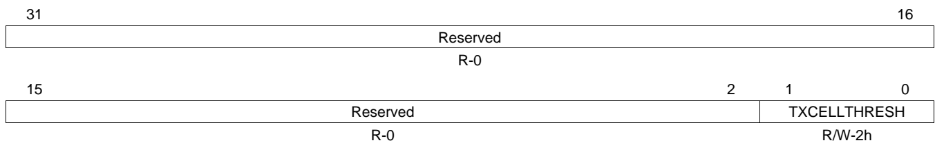
Figure 70. FIFO Control Register (FIFOCONTROL)
