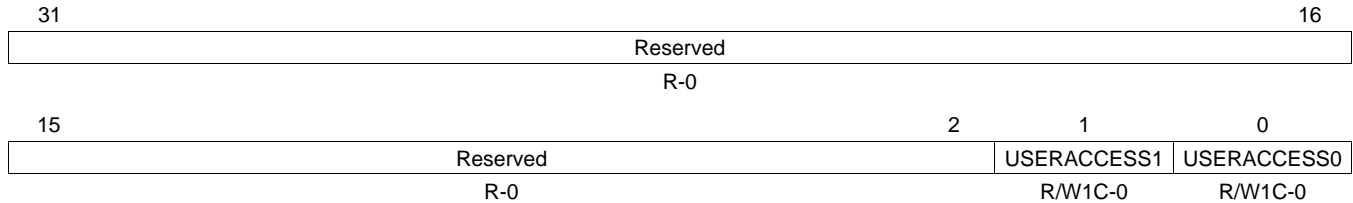
Figure 31. MDIO User Command Complete Interrupt (Unmasked) Register (USERINTRAW)
