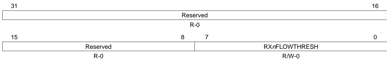
Figure 65. Receive Channel n Flow Control Threshold Register (RX n FLOWTHRESH)
