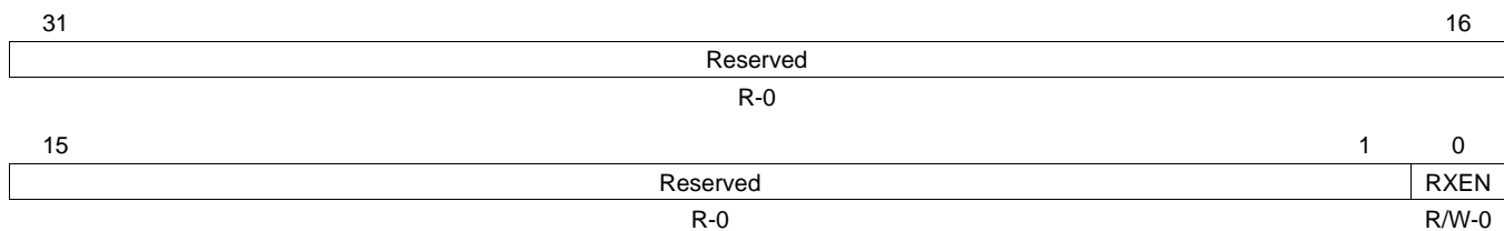
Figure 43. Receive Control Register (RXCONTROL)
