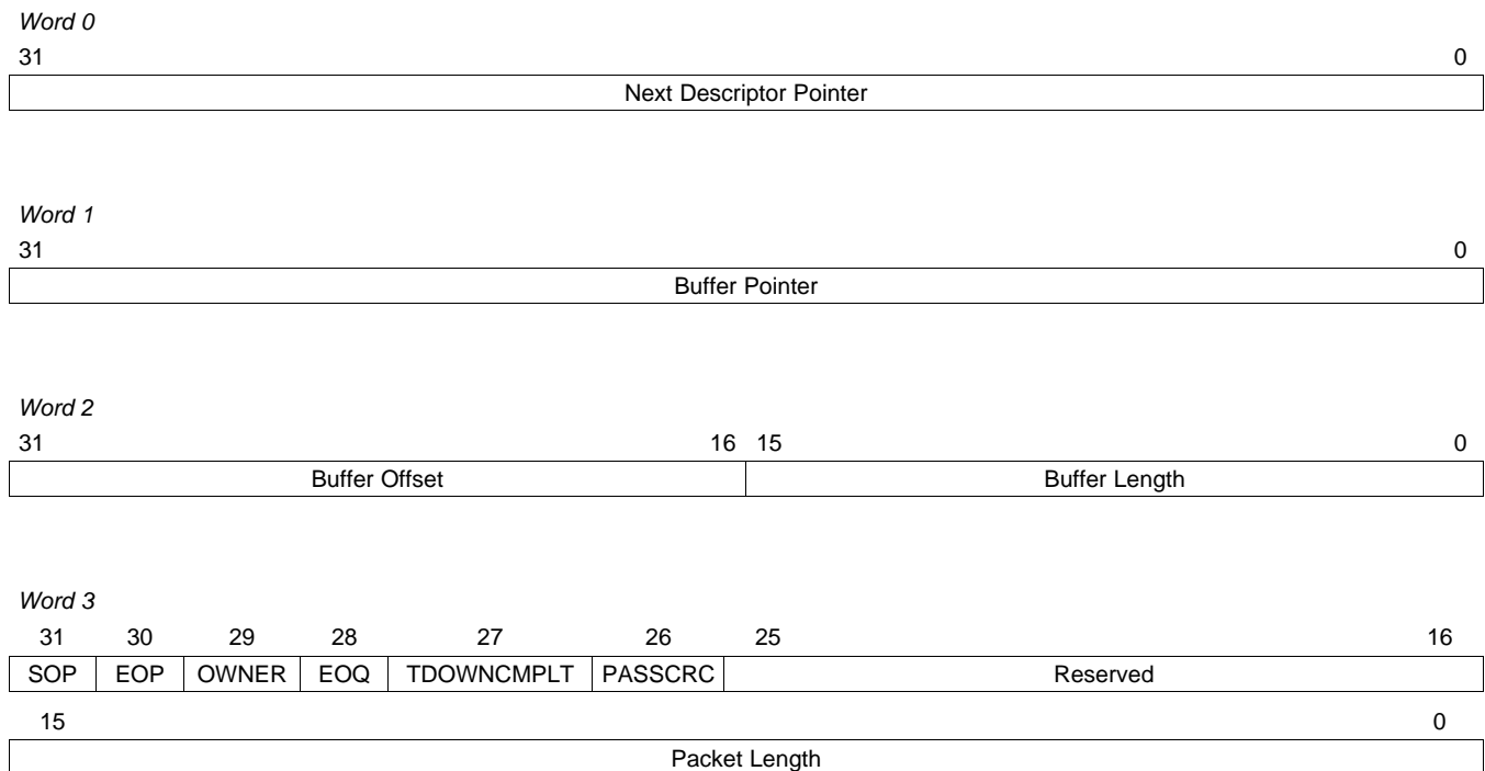
Figure 7. Transmit Buffer Descriptor Format
