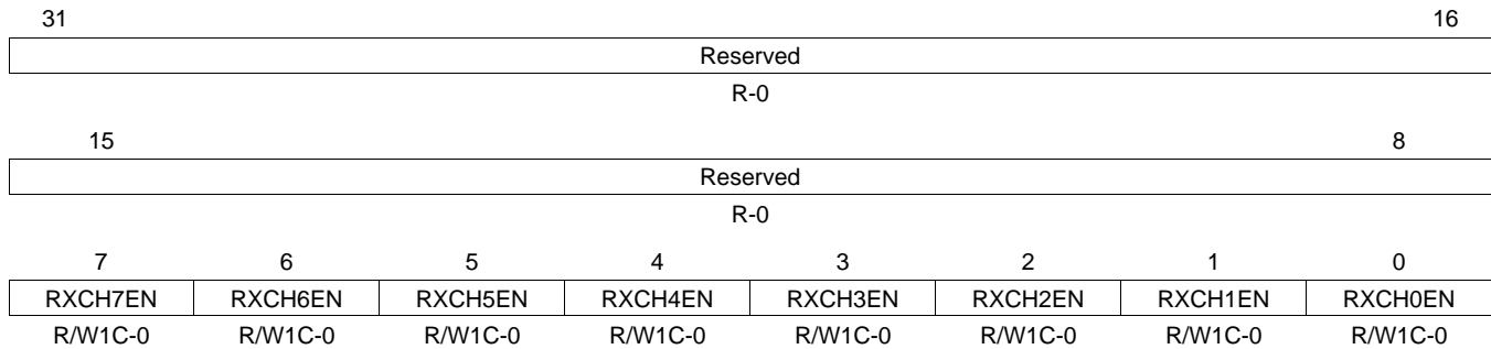
Figure 61. Receive Unicast Clear Register (RXUNICASTCLEAR)
