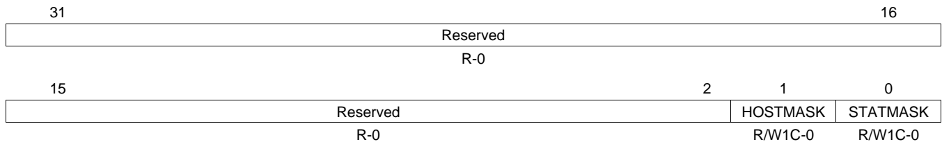
Figure 58. MAC Interrupt Mask Clear Register (MACINTMASKCLEAR)
