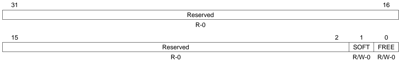
Figure 69. Emulation Control Register (EMCONTROL)
