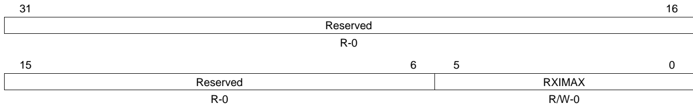
Figure 23. EMAC Control Module Interrupt Core 0-2 Receive Interrupts Per Millisecond Register (CnRXIMAX)
