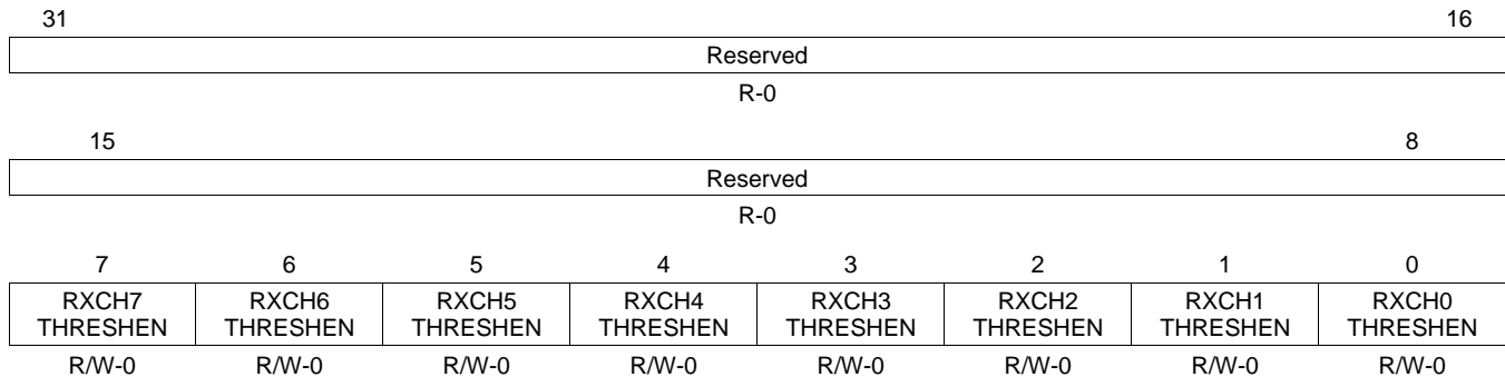
Figure 15. EMAC Control Module Interrupt Core 0-2 Receive Threshold Interrupt Enable Register (CnRXTHRESHEN)
