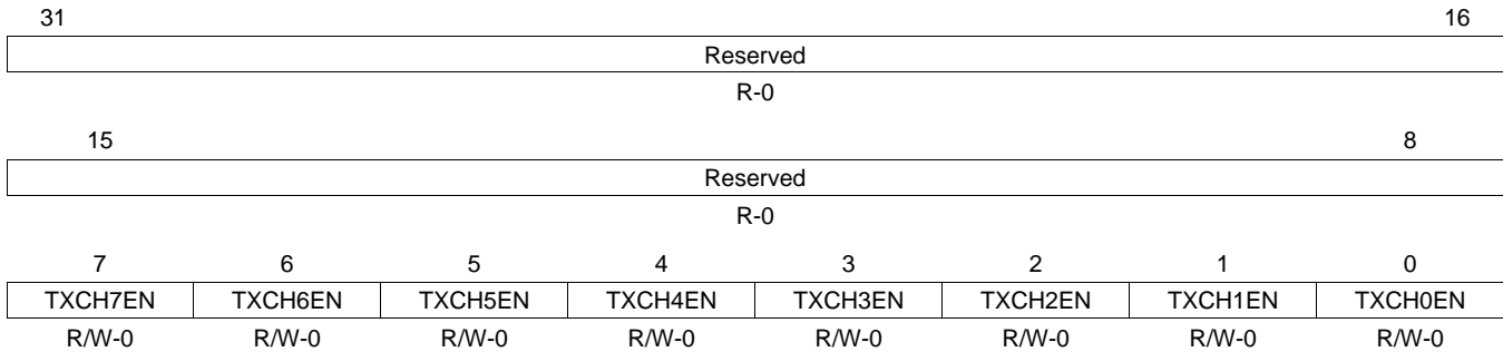
Figure 17. EMAC Control Module Interrupt Core 0-2 Transmit Interrupt Enable Register (CnTXEN)
