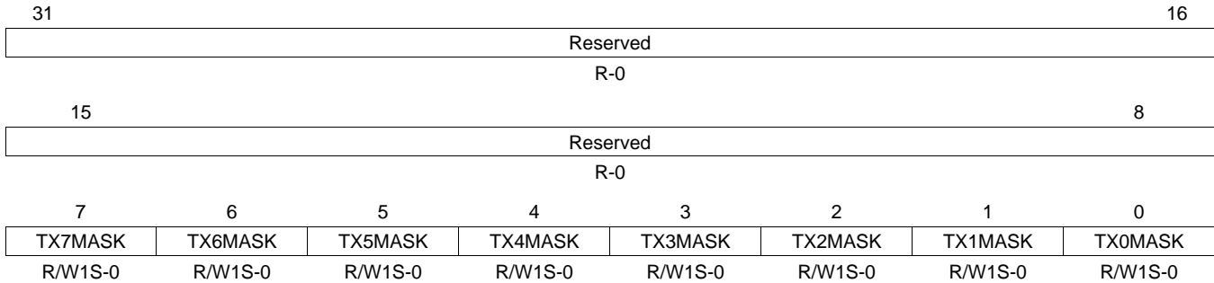
Figure 47. Transmit Interrupt Mask Set Register (TXINTMASKSET)
