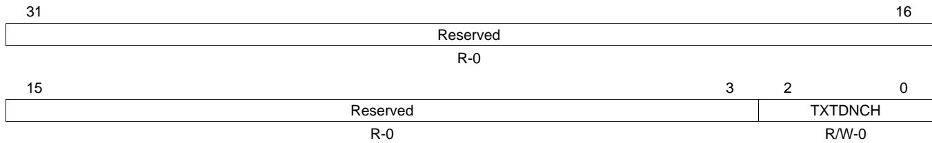
Figure 41. Transmit Teardown Register (TXTEARDOWN)
