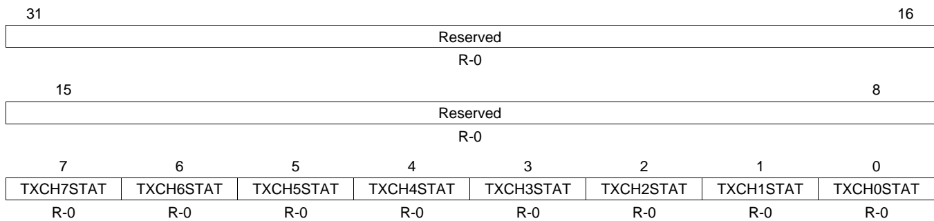
Figure 21. EMAC Control Module Interrupt Core 0-2 Transmit Interrupt Status Register (CnTXSTAT)
