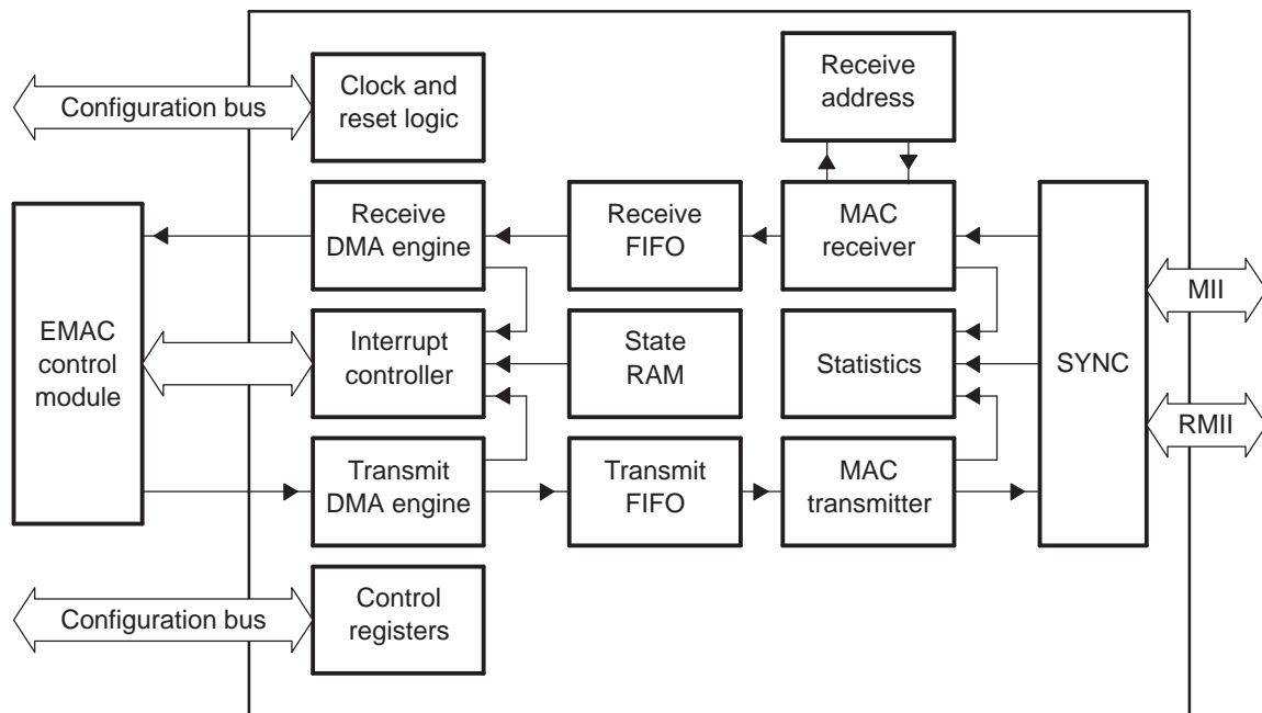
Figure 11. EMAC Module Block Diagram
