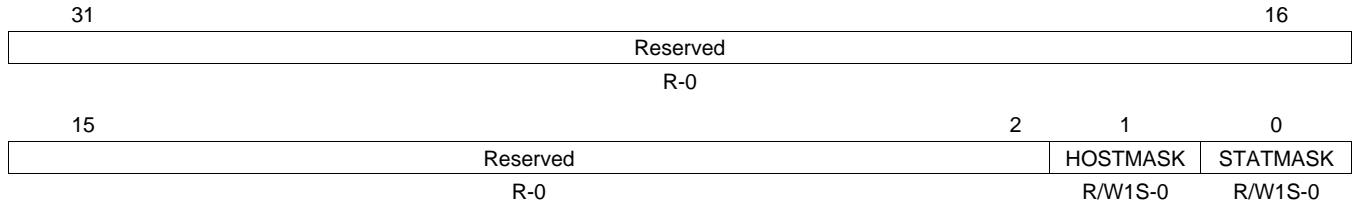
Figure 57. MAC Interrupt Mask Set Register (MACINTMASKSET)
