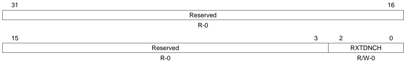
Figure 44. Receive Teardown Register (RXTEARDOWN)
