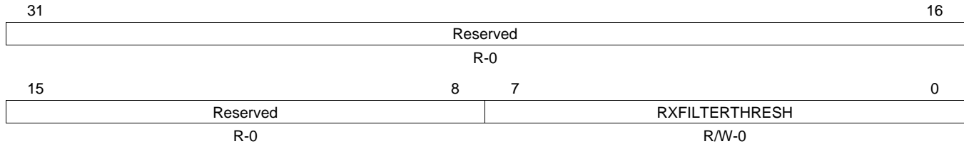
Figure 64. Receive Filter Low Priority Frame Threshold Register (RXFILTERLOWTHRESH)
