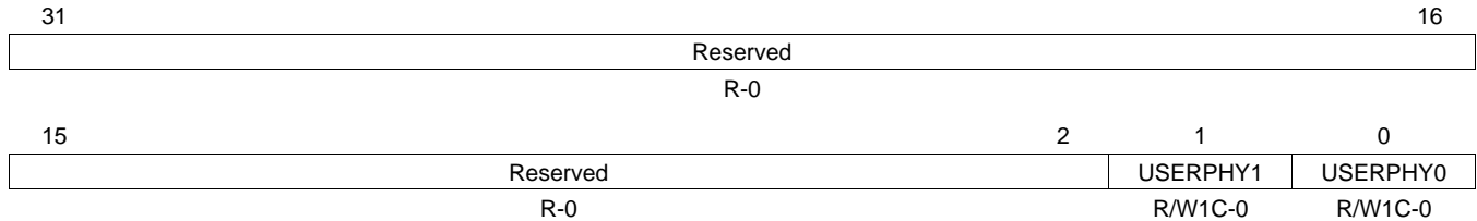
Figure 29. MDIO Link Status Change Interrupt (Unmasked) Register (LINKINTRAW)
