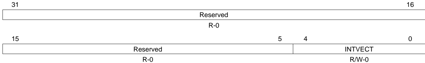
Figure 50. MAC End Of Interrupt Vector Register (MACEOIVECTOR)
