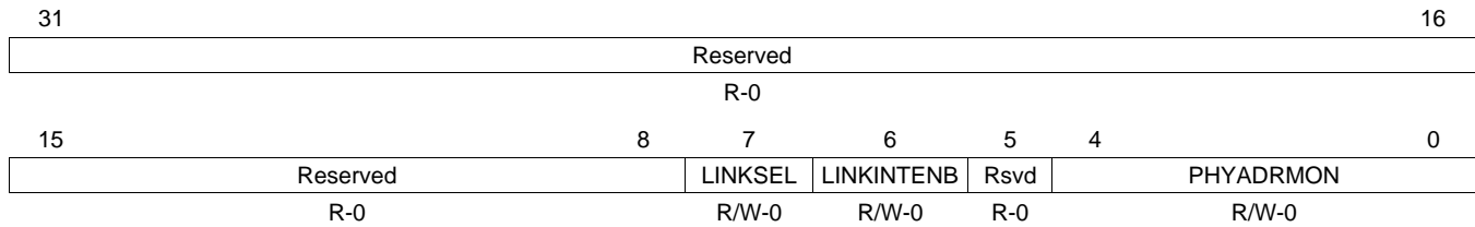
Figure 38. MDIO User PHY Select Register 1 (USERPHYSEL1)
