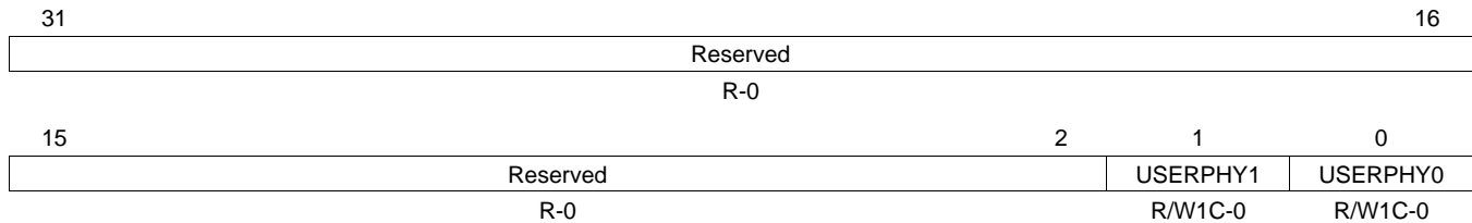
Figure 30. MDIO Link Status Change Interrupt (Masked) Register (LINKINTMASKED)
