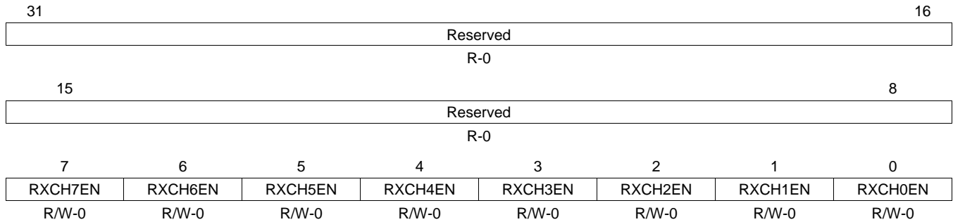
Figure 16. EMAC Control Module Interrupt Core 0-2 Receive Interrupt Enable Register (CnRXEN)
