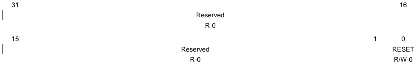
Figure 13. EMAC Control Module Software Reset Register (SOFTRESET)
