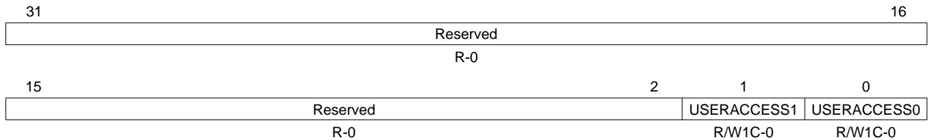
Figure 32. MDIO User Command Complete Interrupt (Masked) Register (USERINTMASKED)
