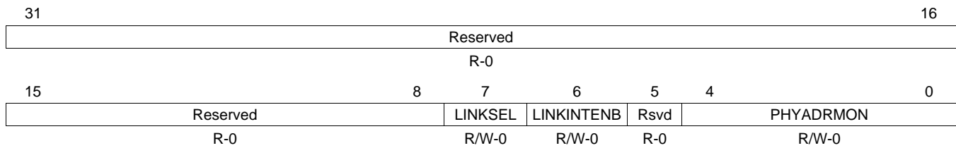
Figure 36. MDIO User PHY Select Register 0 (USERPHYSEL0)
