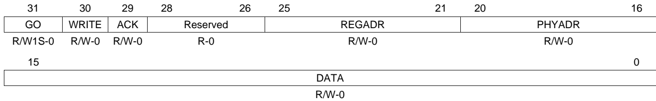
Figure 37. MDIO User Access Register 1 (USERACCESS1)
