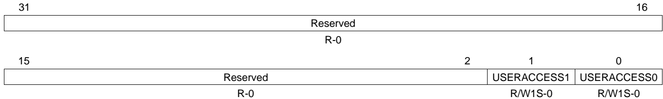
Figure 33. MDIO User Command Complete Interrupt Mask Set Register (USERINTMASKSET)
