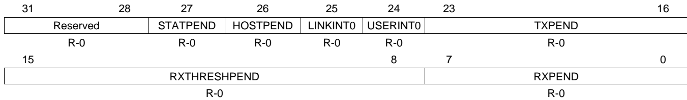
Figure 49. MAC Input Vector Register (MACINVECTOR)
