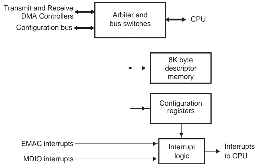
Figure 9. EMAC Control Module Block Diagram
