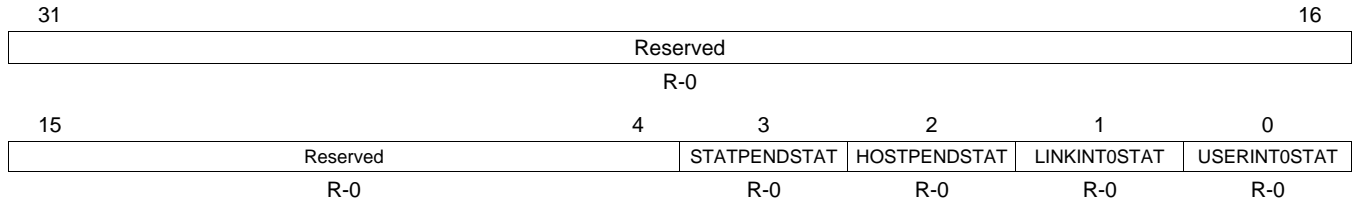
Figure 22. EMAC Control Module Interrupt Core 0-2 Miscellaneous Interrupt Status Register (CnMISCSTAT)
