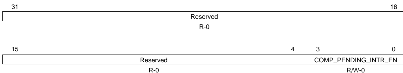
Figure 39. Receive CPPI Interrupt Enable Set Register (RCPPIENSETR)
