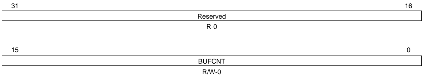
Figure 42. Receive Buffer Count 1 Register (RBUFCNT1)
