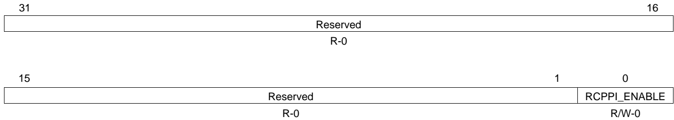
Figure 36. Receive CPPI Control Register (RCPPICR)
