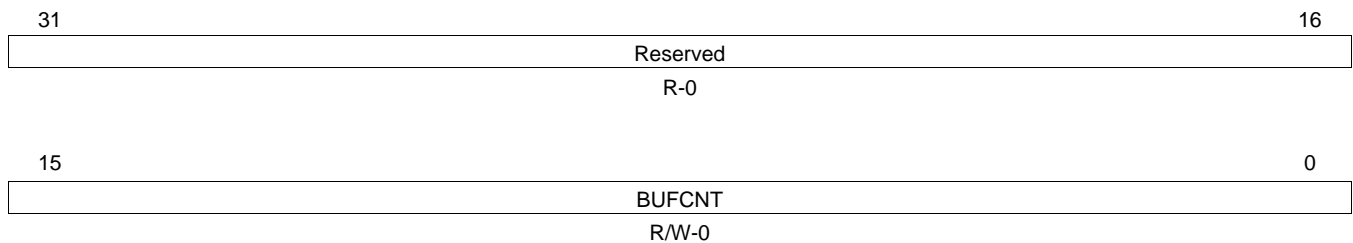
Figure 41. Receive Buffer Count 0 Register (RBUFCNT0)
