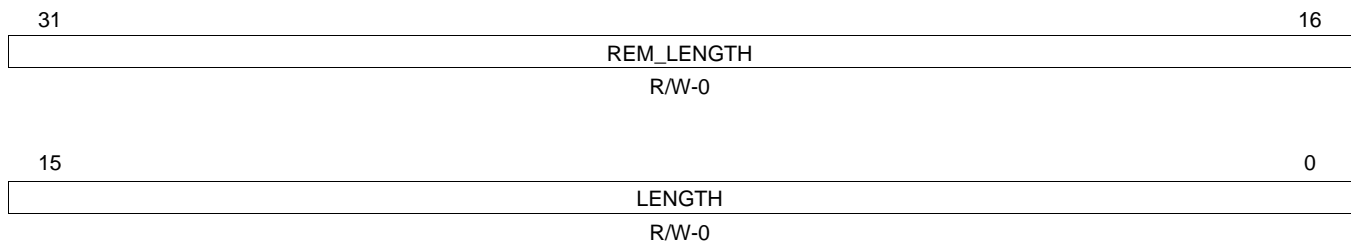
Figure 50. Transmit CPPI DMA State Word 5 (TCPPIDMASTATEW5)
