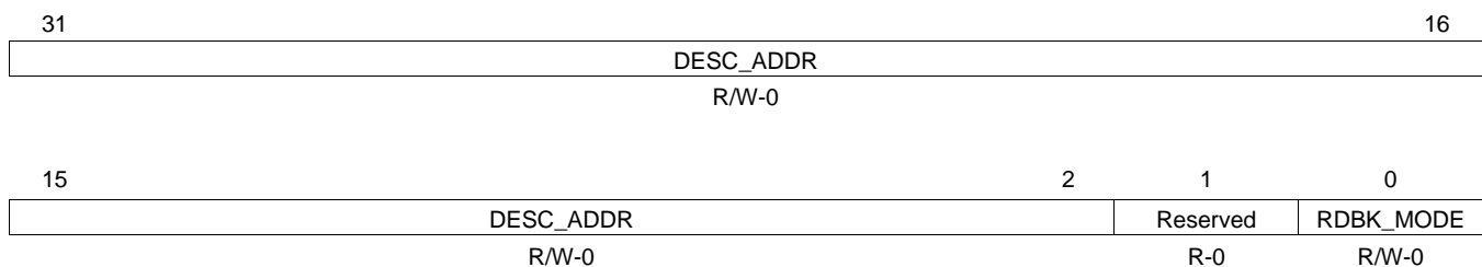
Figure 59. Receive CPPI Completion Pointer (RCPPICOMPTR)
