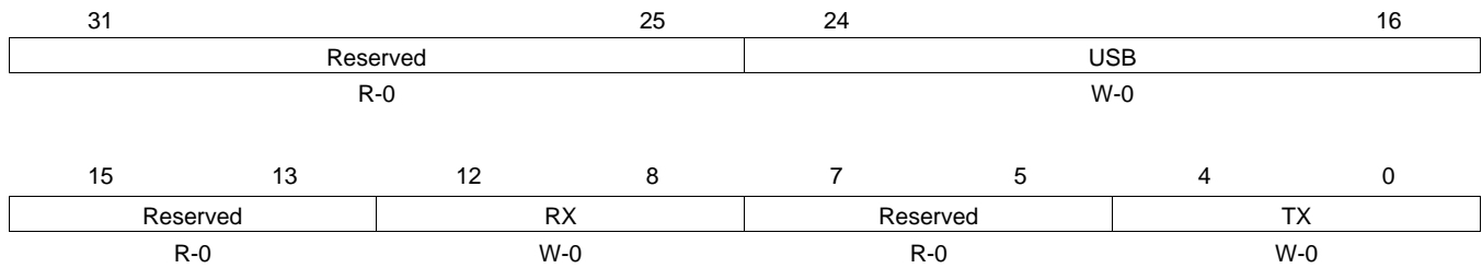
Figure 22. USB Interrupt Source Clear Register (INTCLRR)
