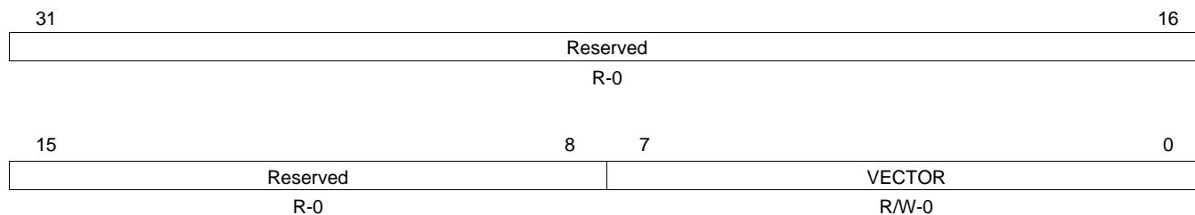
Figure 31. CPPI DMA End of Interrupt Register (CPPIEOIR)
