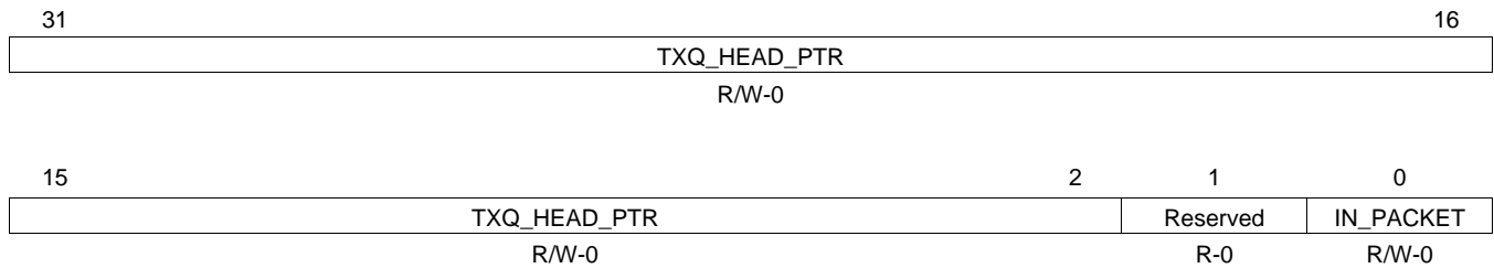
Figure 45. Transmit CPPI DMA State Word 0 (TCPPIDMASTATEW0)
