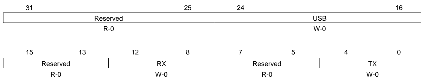
Figure 25. USB Interrupt Mask Clear Register (INTMSKCLRR)
