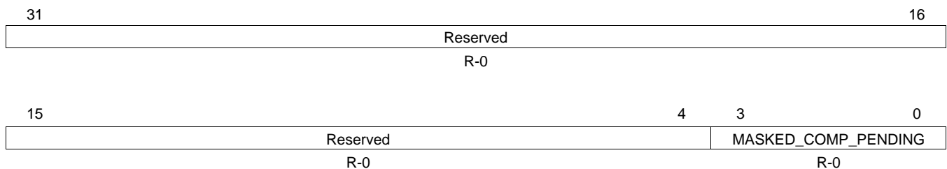
Figure 37. Receive CPPI Masked Status Register (RCPPIMSKSR)
