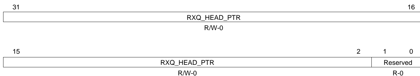
Figure 53. Receive CPPI DMA State Word 1 (RCPPIIDMASTATEW1)
