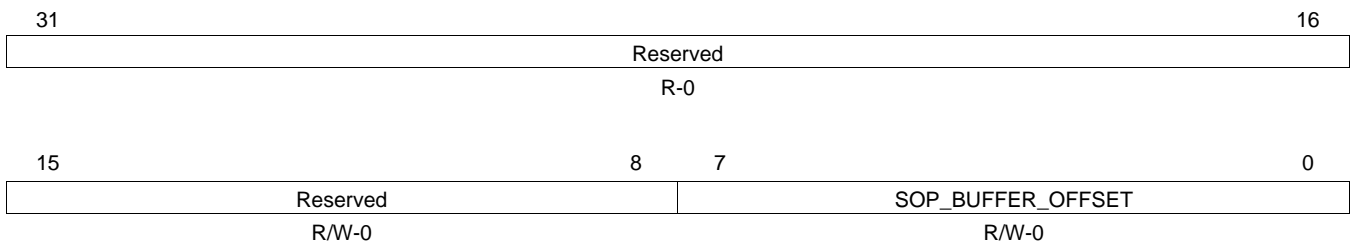
Figure 52. Receive CPPI DMA State Word 0 (RCPPIIDMASTATEW0)
