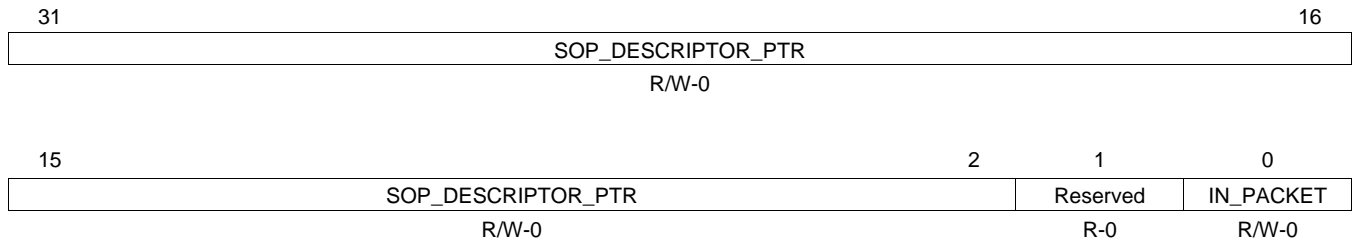
Figure 46. Transmit CPPI DMA State Word 1 (TCPPIDMASTATEW1)
