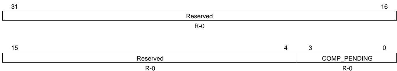
Figure 33. Transmit CPPI Raw Status Register (TCPPIRAWSR)
