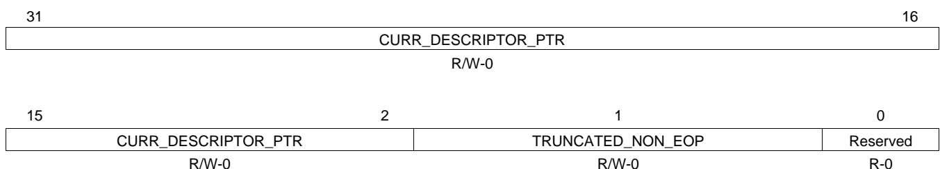
Figure 47. Transmit CPPI DMA State Word 2 (TCPPIDMASTATEW2)
