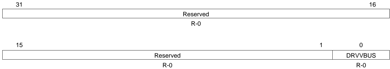
Figure 17. Status Register (STATR)
