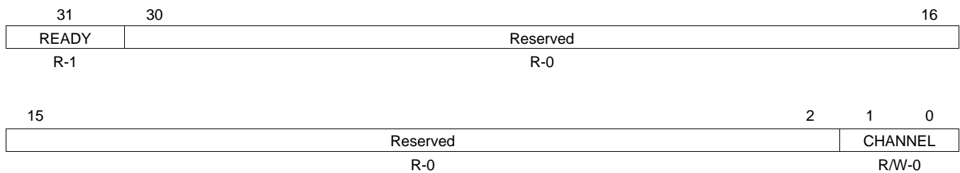
Figure 30. Transmit CPPI Teardown Register (TCPPI TDR)
