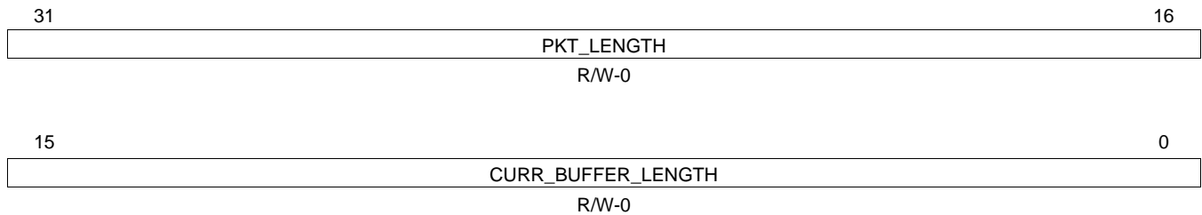
Figure 57. Receive CPPI DMA State Word 5 (RCPPIDMASTATEW5)
