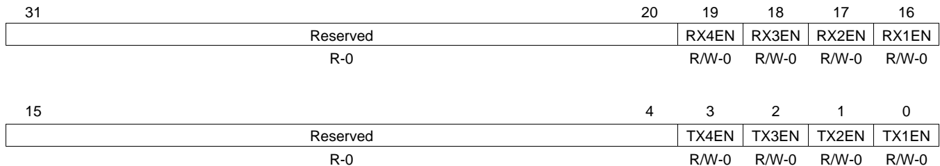
Figure 18. RNDIS Register (RNDISR)
