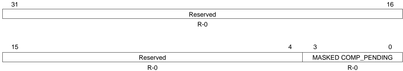
Figure 32. Transmit CPPI Masked Status Register (TCPPIMSKSR)
