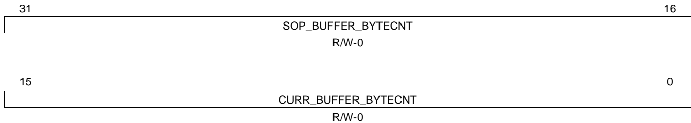
Figure 58. Receive CPPI DMA State Word 6 (RCPPIDMASTATEW6)
