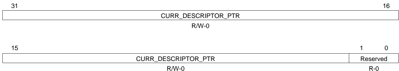
Figure 55. Receive CPPI DMA State Word 3 (RCPPIDMASTATEW3)
