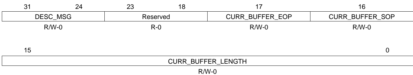
Figure 49. Transmit CPPI DMA State Word 4 (TCPPIDMASTATEW4)
