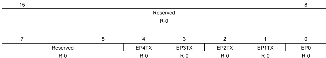
Figure 62. Interrupt Register for Endpoint 0 Plus Tx Endpoints 1 to 4 (INTRTX)
