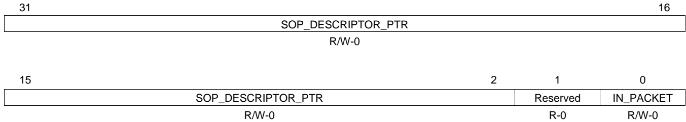
Figure 54. Receive CPPI DMA State Word 2 (RCPPIDMASTATEW2)
