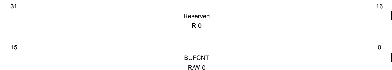
Figure 43. Receive Buffer Count 2 Register (RBUFCNT2)
