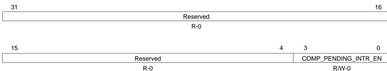
Figure 35. Transmit CPPI Interrupt Enable Clear Register (TCPPIIENCLR)
