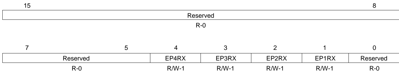
Figure 65. Interrupt Enable Register for INTRRX (INTRRXE)
