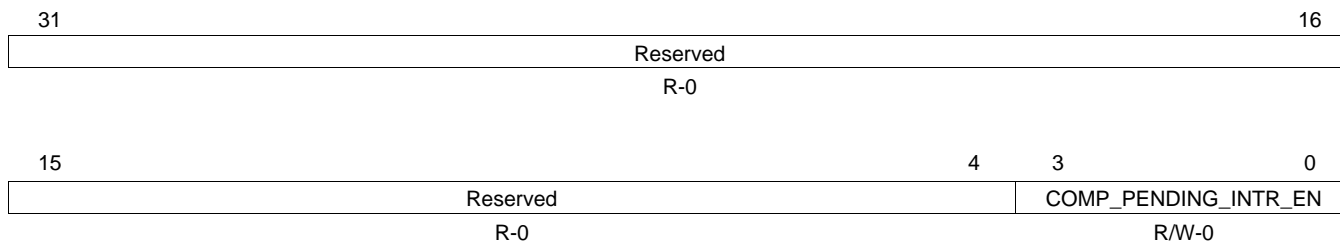
Figure 34. Transmit CPPI Interrupt Enable Set Register (TCPPIIENSETR)
