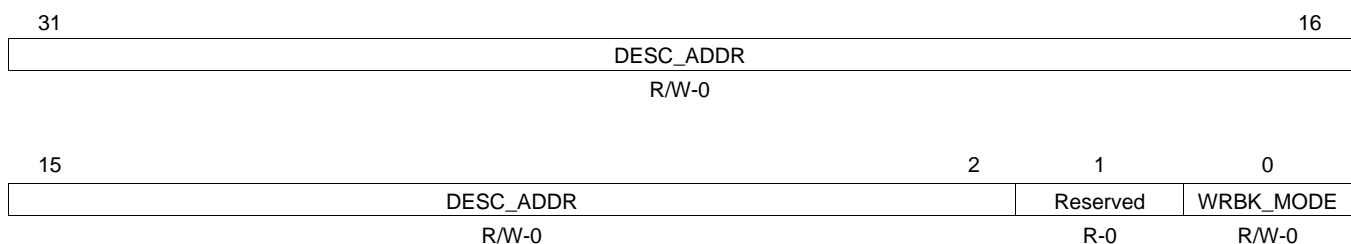
Figure 51. Transmit CPPI Completion Pointer (TCPPICOMPTR)
