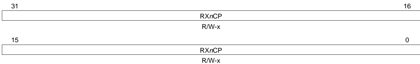
Figure 74. Receive Channel n Completion Pointer Register (RX n CP)
