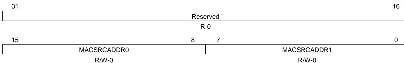
Figure 60. MAC Source Address Low Bytes Register (MACSRCADDRLO)
