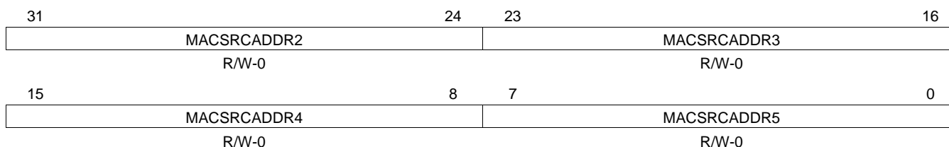
Figure 61. MAC Source Address High Bytes Register (MACSRCADDRHI)
