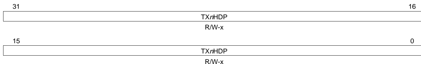
Figure 71. Transmit Channel n DMA Head Descriptor Pointer Register (TXnHDP)
