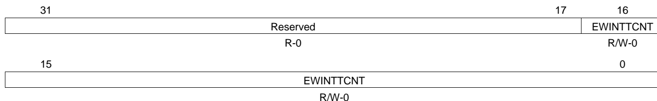
Figure 12. EMAC Control Module Interrupt Timer Count Register (EWINTTCNT)
