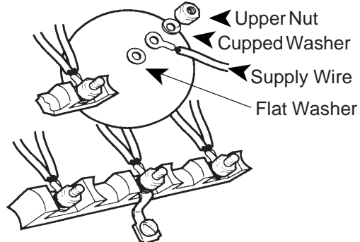
FIG. 9 Conductor Securement
