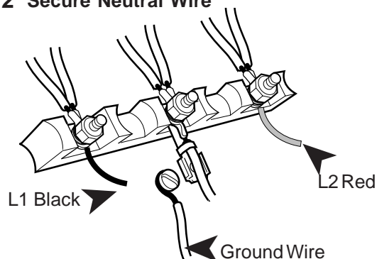
FIG. 12 Secure Neutral Wire
