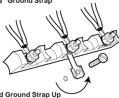
FIG. 11 Ground Strap
