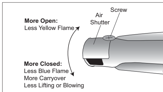
FIG. 15 Air Shutter Adjustment (if necessary)
