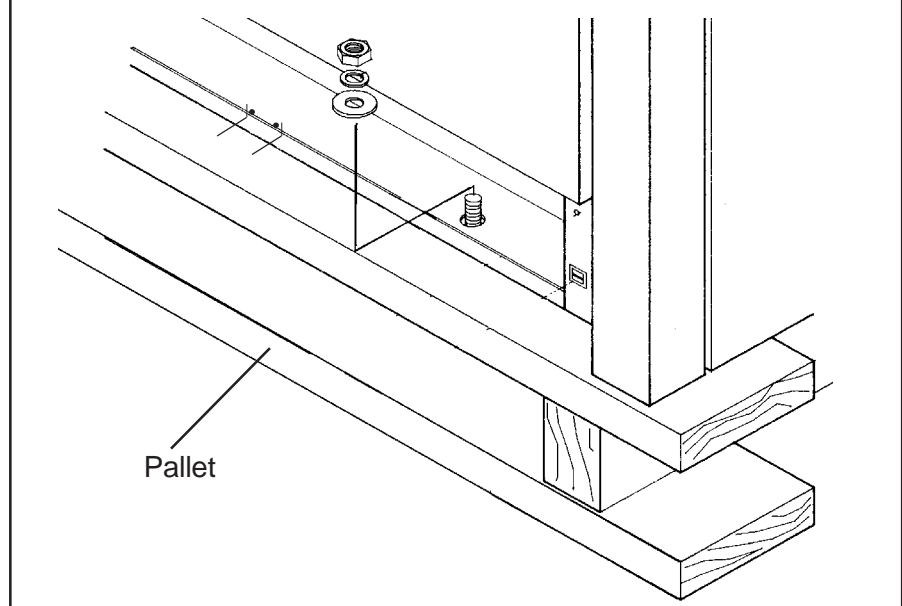
FIG. 4 – Removal of the Four (4) Shipping Bolts
