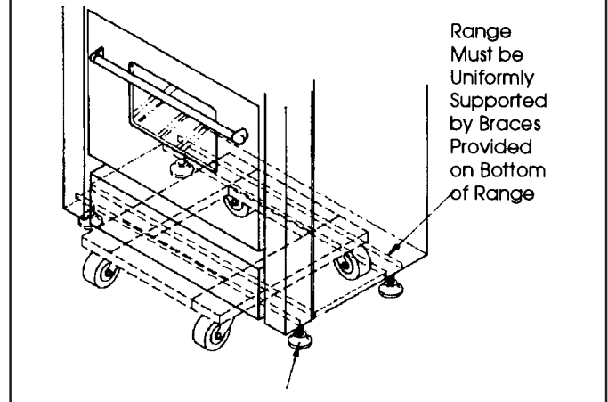
FIG. 5- Dolly Positioning
