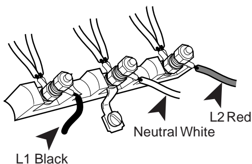
FIG. 11 Ground Strap
