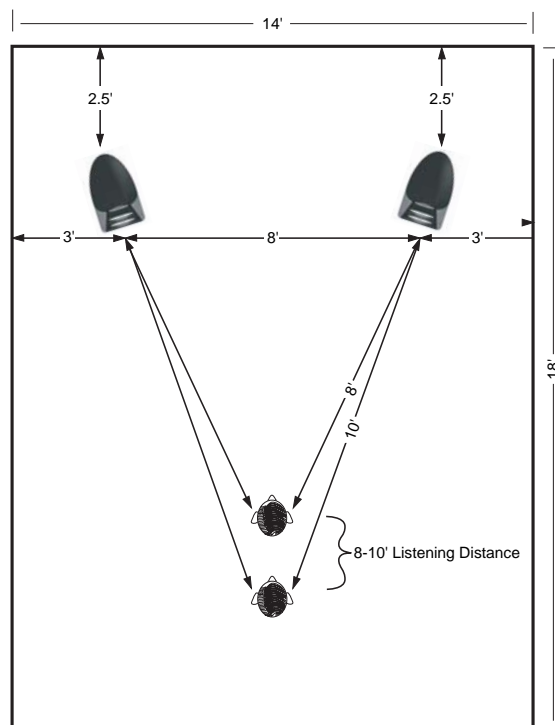
Figure 3. Average listening room
