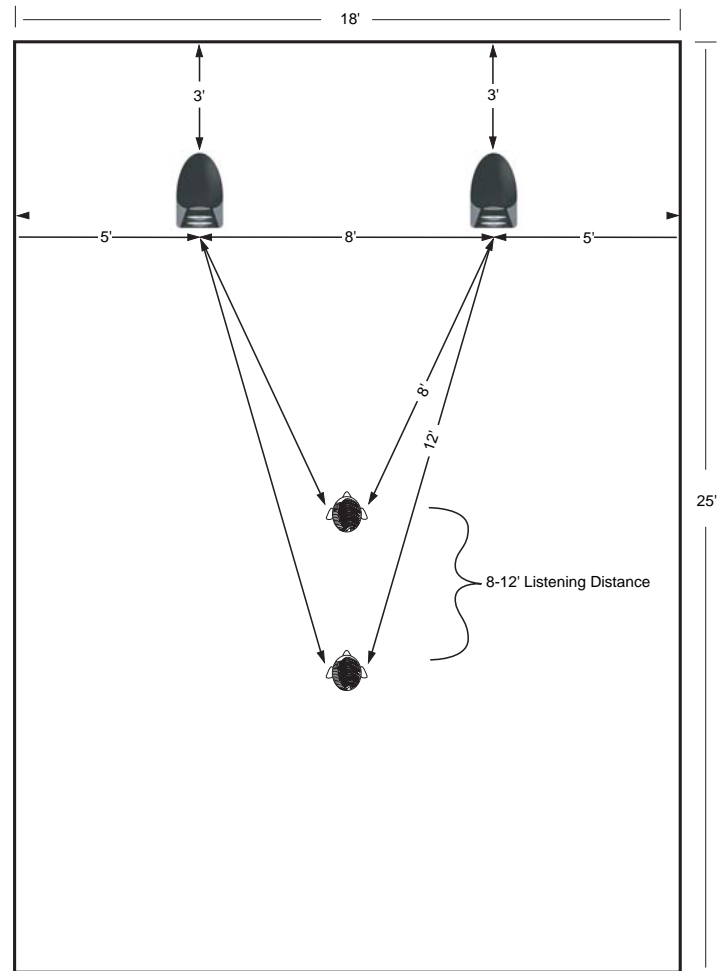
Figure 5. Large listening room speaker placement
