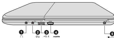
Figure 2-3 The right side of the computer
