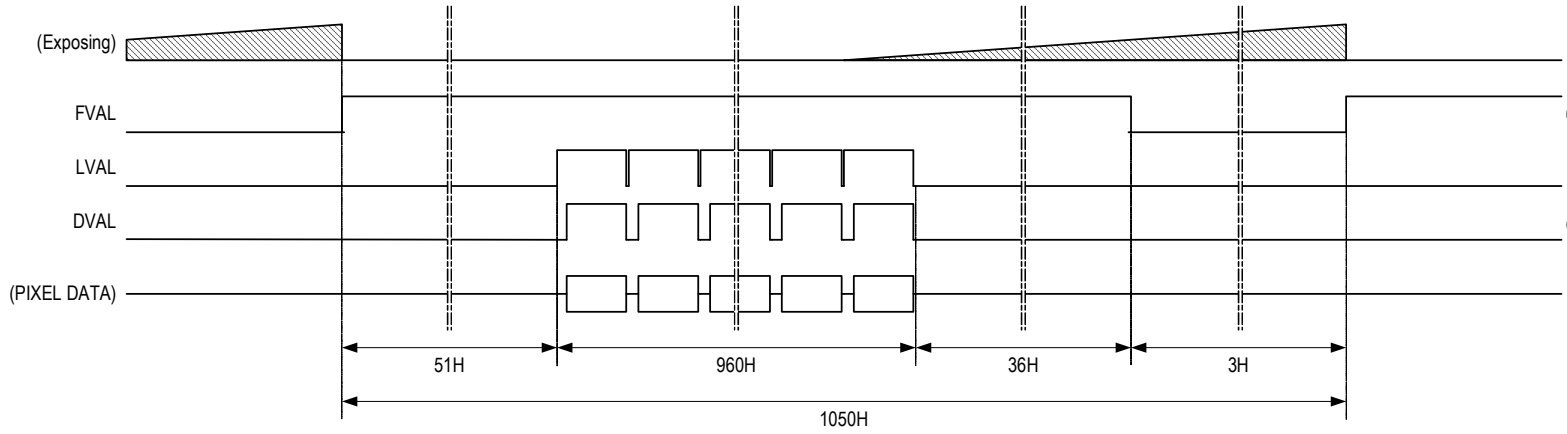
(1) SXGA output timing
