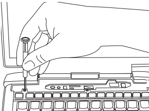
Removing the left keyboard screw
