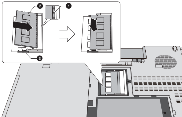
Figure 4-10 Seating the memory module
