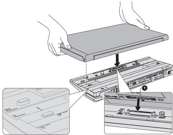
Figure 4-18 Aligning your computer with the Port Replicator
