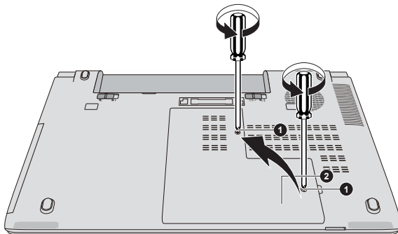
Figure 4-9 Removing the memory module cover
