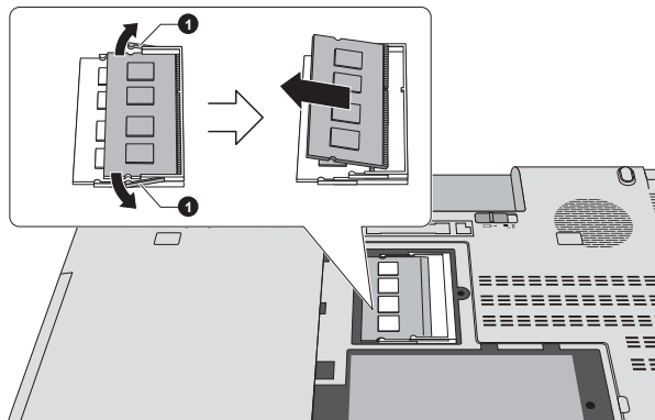
Figure 4-12 Removing the memory module
