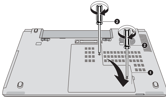
Figure 4-11 Seating the memory module cover
