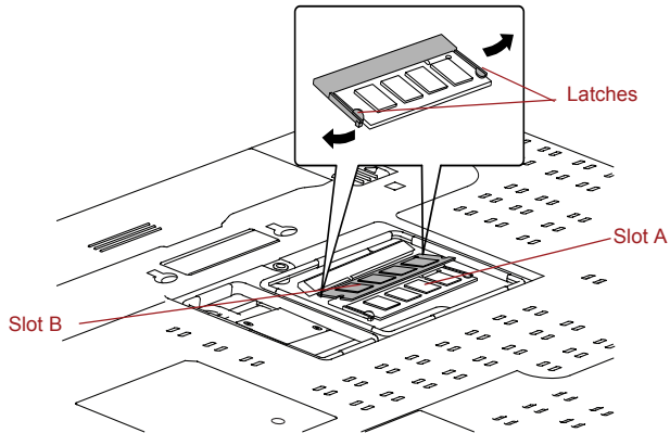
Figure 3-9 Removing the memory module
