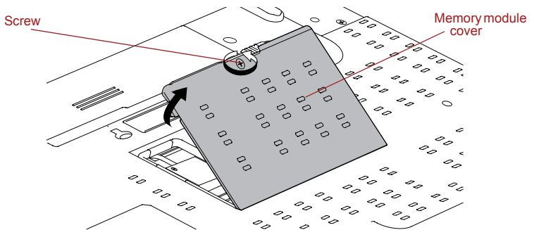
Figure 3-6 Removing the memory module cover
