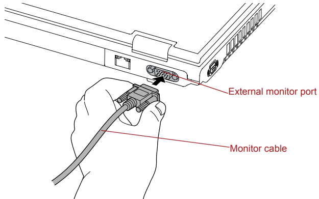
Figure 3-10 Connecting the monitor cable to the external monitor port
