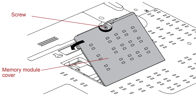
Figure 3-8 Seating the memory module cover
