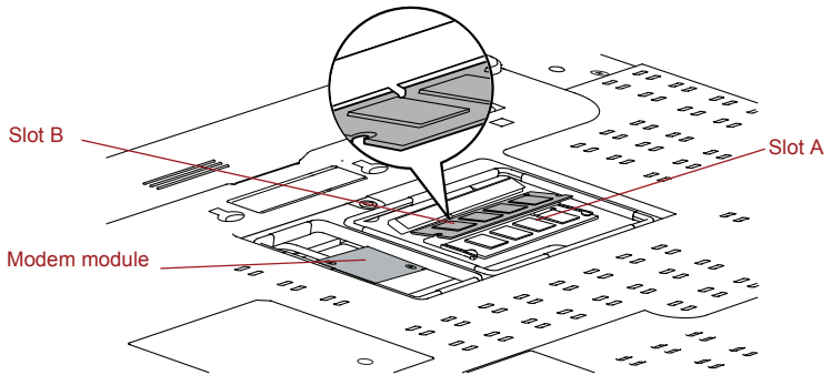
Figure 3-7 Seating the memory module
