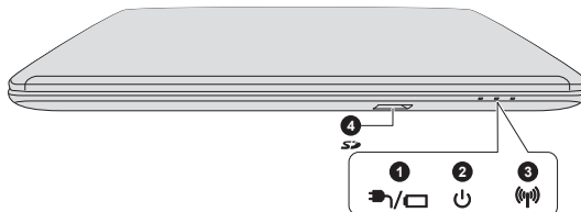
Figure 3-2 Front of the computer with display panel closed (X70-A)
