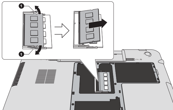
Figure 4-16 Removing the memory module
