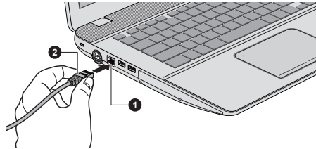
Figure 4-12 Connecting the LAN cable
