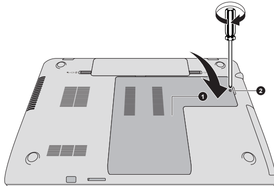
Figure 4-15 Seating the memory module cover
