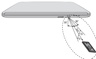
Figure 4-3 Operational range of the remote controller
