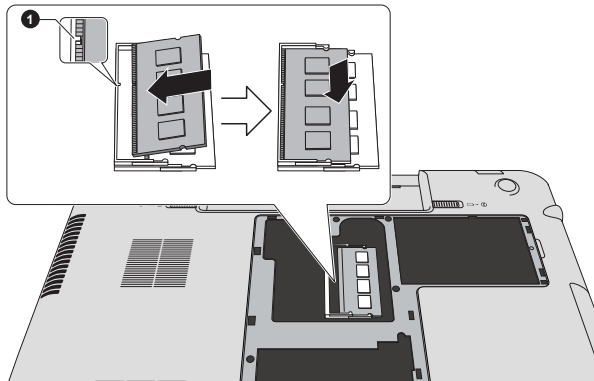
Figure 4-14 Seating the memory module
