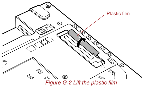
Figure G-2 Lift the plastic film
