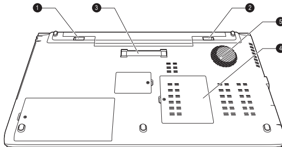
Figure 2-5 The underside of the computer (R950)
