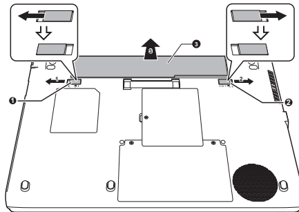
Figure 5-1 Releasing the battery pack (R940)
