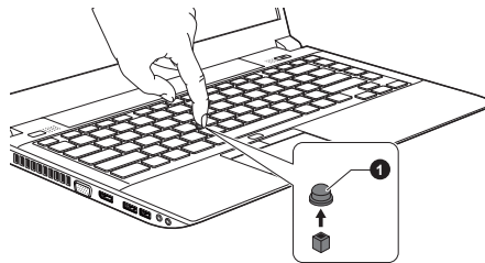
Figure 3-2 Removing the AccuPoint cap (R940)
