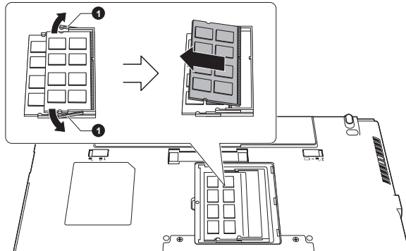
Figure 3-15 Removing the memory module (R940)
