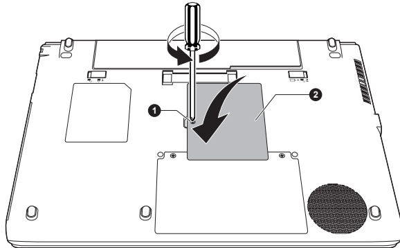
Figure 3-14 Seating the memory module cover (R940)
