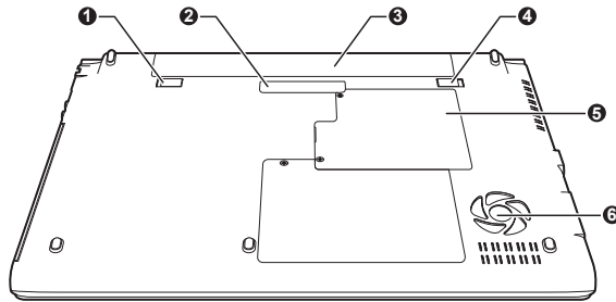
Figure 2-17 The underside of the computer (R930)
