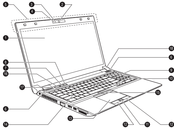
Figure 2-6 The front of the computer with the display panel open (R950)
