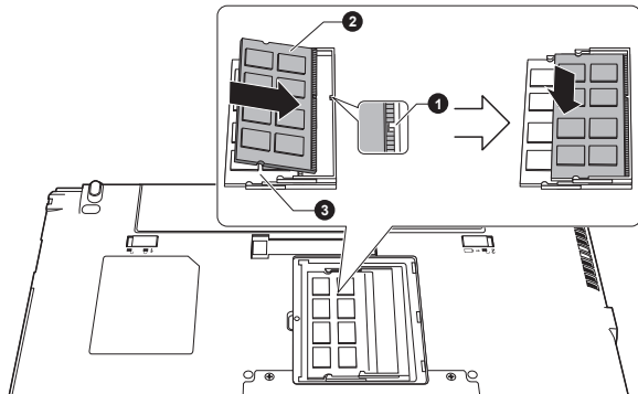
Figure 3-13 Seating the memory module (R940)
