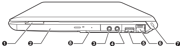
Figure 2-15 The right side of the computer (R930)
